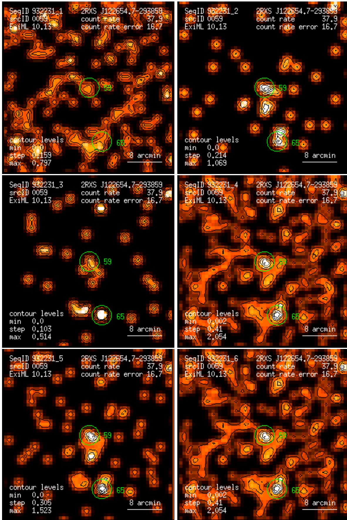
Figure 59: RASS 932231: detection 0059: band rate images, Gaussian filter: (1) PSPC channels 11 – 41, (2) 52 – 90, (3) 91 – 201, (4) 11 – 235, (5) 52 – 201, (6) 11 – 201. Broad band rates in counts/ks. Band rate contour levels in counts/ks/arcmin 2 .
