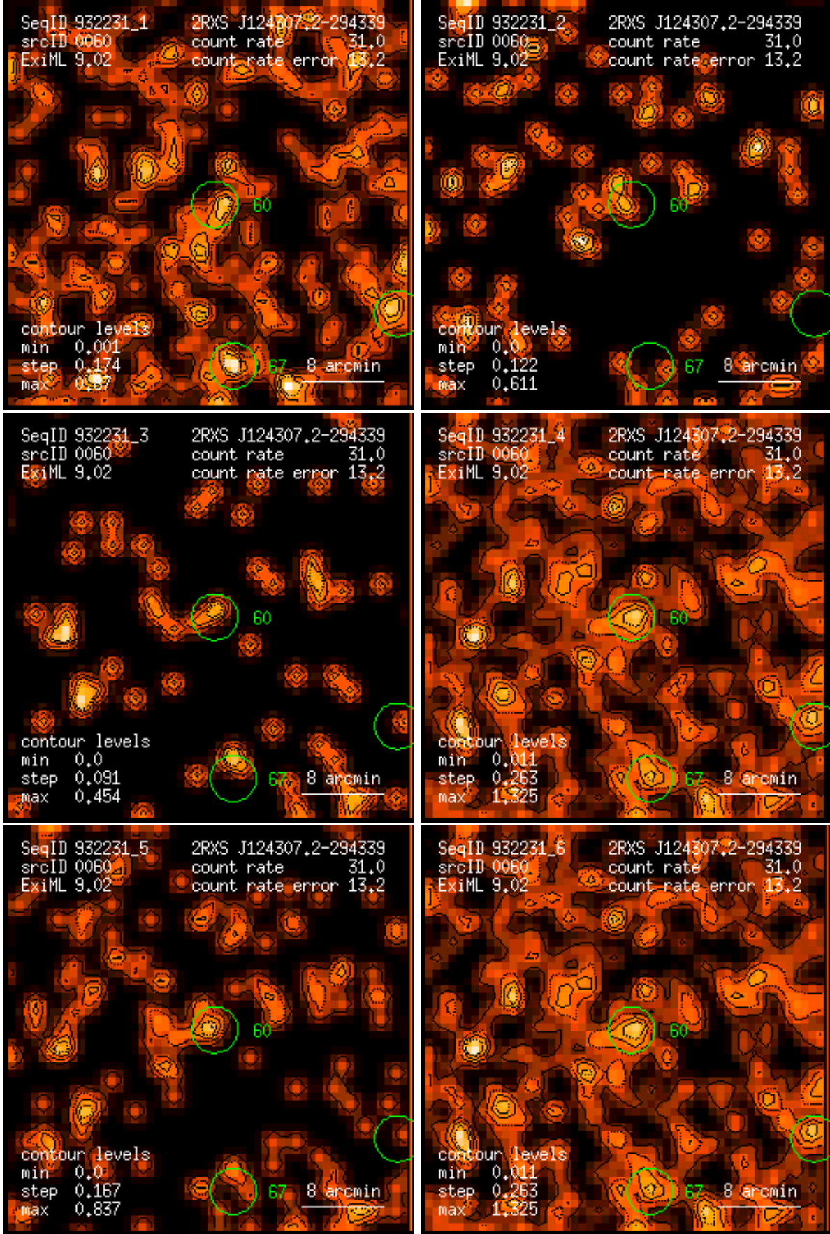
Figure 60: RASS 932231: detection 0060: band rate images, Gaussian filter: (1) PSPC channels 11 – 41, (2) 52 – 90, (3) 91 – 201, (4) 11 – 235, (5) 52 – 201, (6) 11 – 201. Broad band rates in counts/ks. Band rate contour levels in counts/ks/arcmin 2 .
