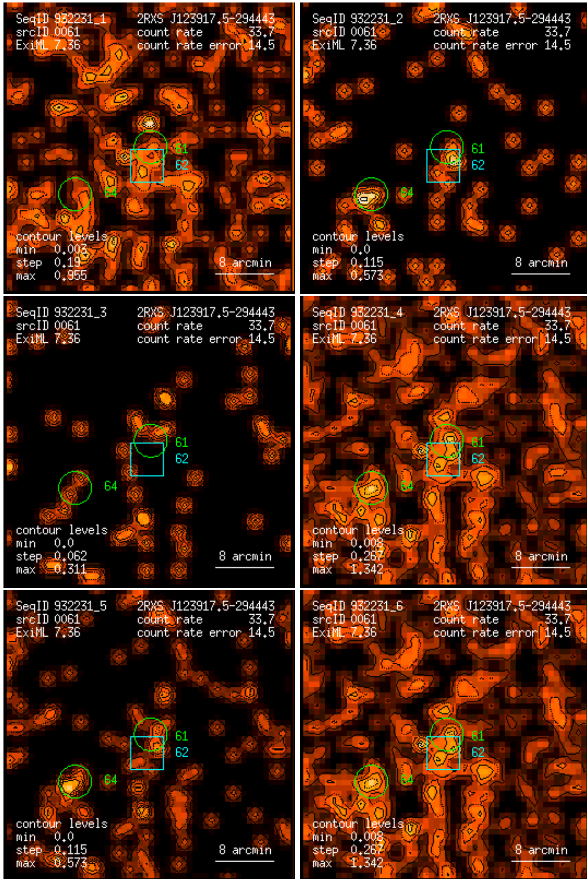
Figure 61: RASS 932231: detection 0061: band rate images, Gaussian filter: (1) PSPC channels 11 – 41, (2) 52 – 90, (3) 91 – 201, (4) 11 – 235, (5) 52 – 201, (6) 11 – 201. Broad band rates in counts/ks. Band rate contour levels in counts/ks/arcmin 2 .
