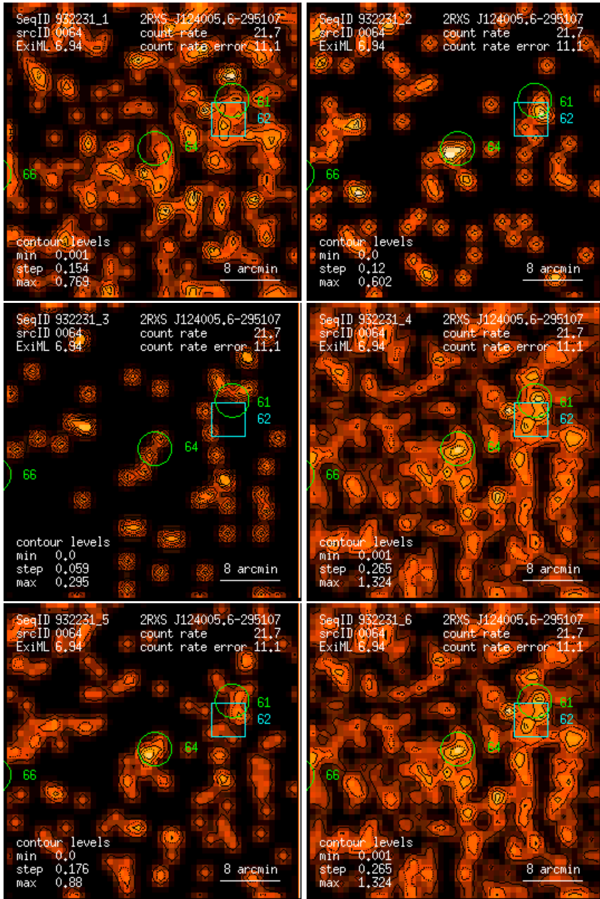
Figure 64: RASS 932231: detection 0064: band rate images, Gaussian filter: (1) PSPC channels 11 – 41, (2) 52 – 90, (3) 91 – 201, (4) 11 – 235, (5) 52 – 201, (6) 11 – 201. Broad band rates in counts/ks. Band rate contour levels in counts/ks/arcmin 2 .
