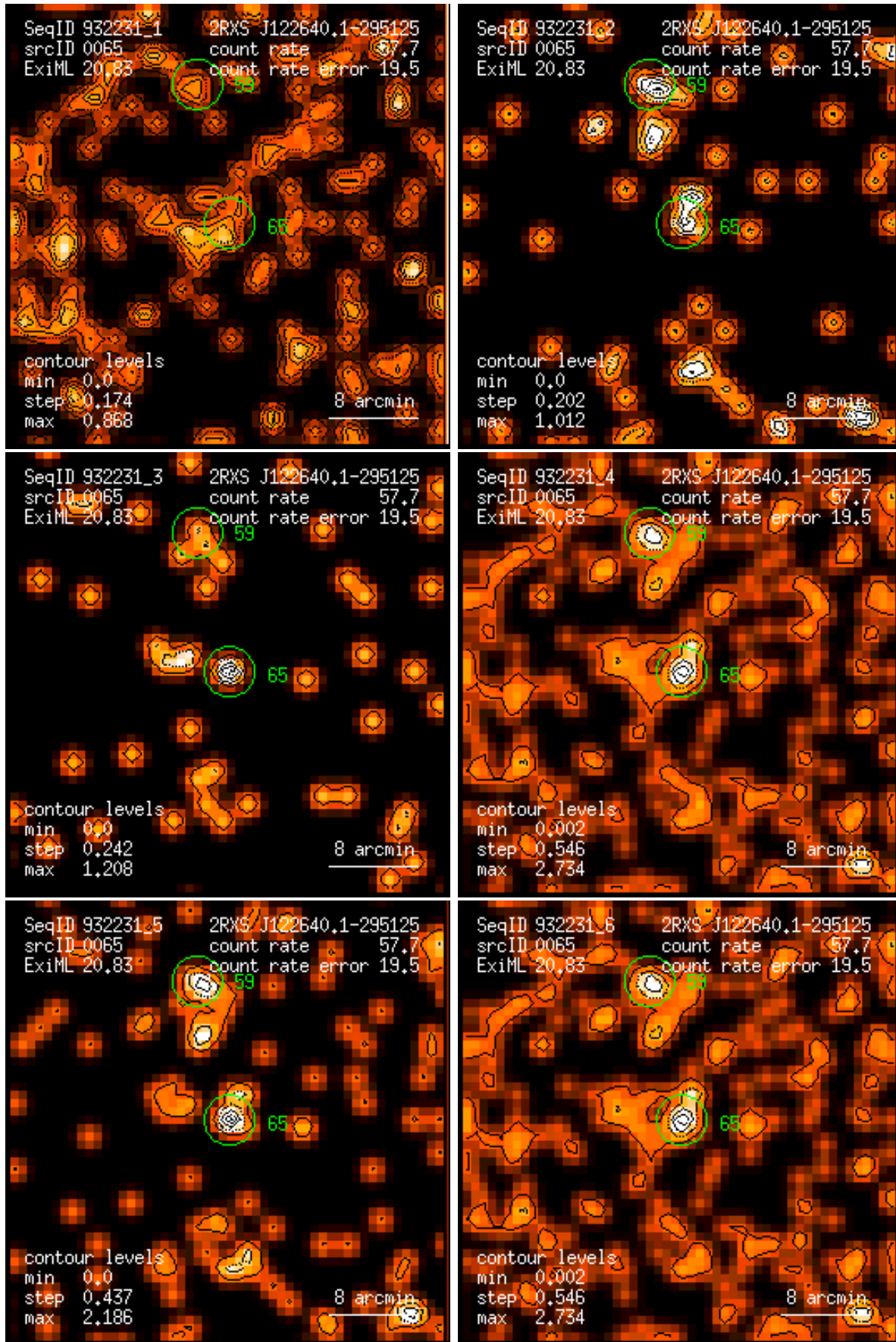
Figure 65: RASS 932231: detection 0065: band rate images, Gaussian filter: (1) PSPC channels 11 – 41, (2) 52 – 90, (3) 91 – 201, (4) 11 – 235, (5) 52 – 201, (6) 11 – 201. Broad band rates in counts/ks. Band rate contour levels in counts/ks/arcmin 2 .
