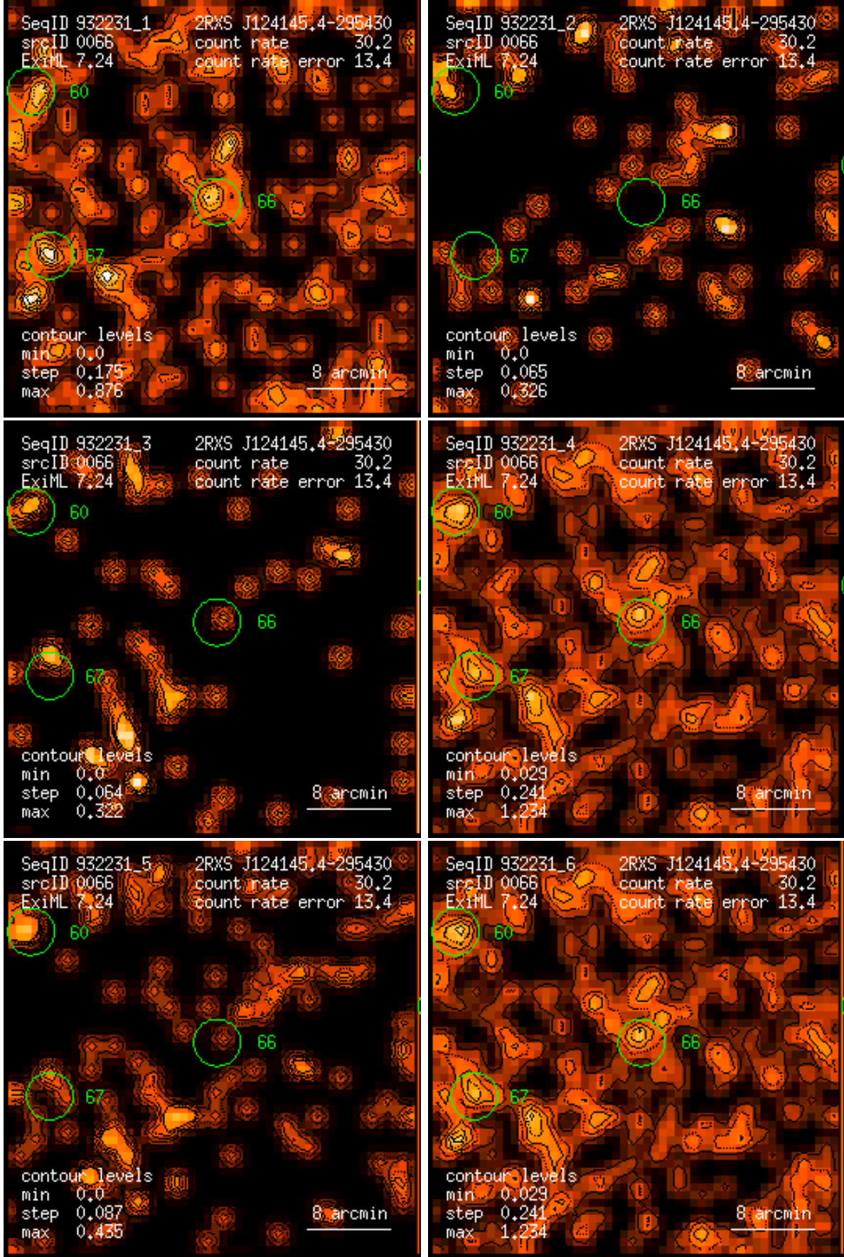
Figure 66: RASS 932231: detection 0066: band rate images, Gaussian filter: (1) PSPC channels 11 – 41, (2) 52 – 90, (3) 91 – 201, (4) 11 – 235, (5) 52 – 201, (6) 11 – 201. Broad band rates in counts/ks. Band rate contour levels in counts/ks/arcmin 2 .
