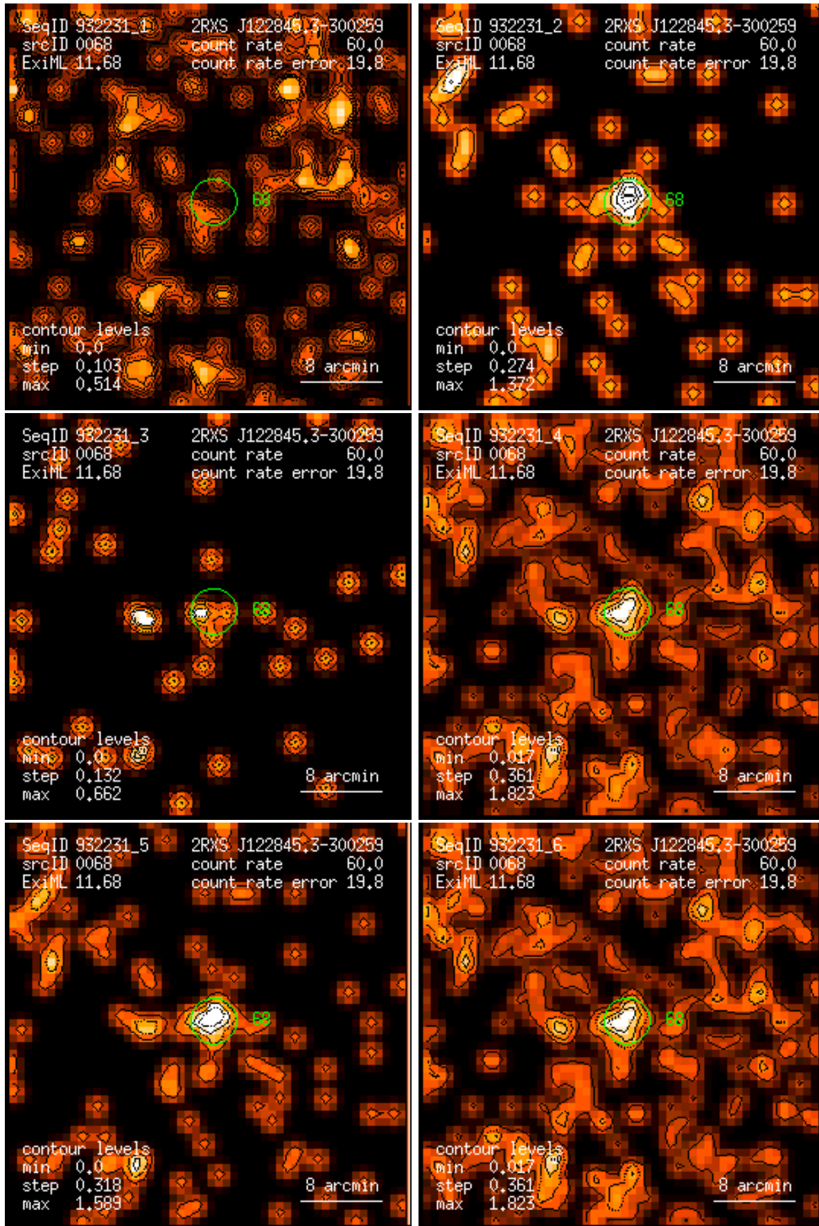
Figure 68: RASS 932231: detection 0068: band rate images, Gaussian filter: (1) PSPC channels 11 – 41, (2) 52 – 90, (3) 91 – 201, (4) 11 – 235, (5) 52 – 201, (6) 11 – 201. Broad band rates in counts/ks. Band rate contour levels in counts/ks/arcmin 2 .
