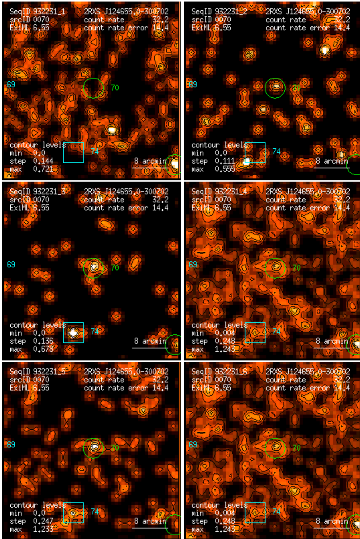
Figure 70: RASS 932231: detection 0070: band rate images, Gaussian filter: (1) PSPC channels 11 – 41, (2) 52 – 90, (3) 91 – 201, (4) 11 – 235, (5) 52 – 201, (6) 11 – 201. Broad band rates in counts/ks. Band rate contour levels in counts/ks/arcmin 2 .
