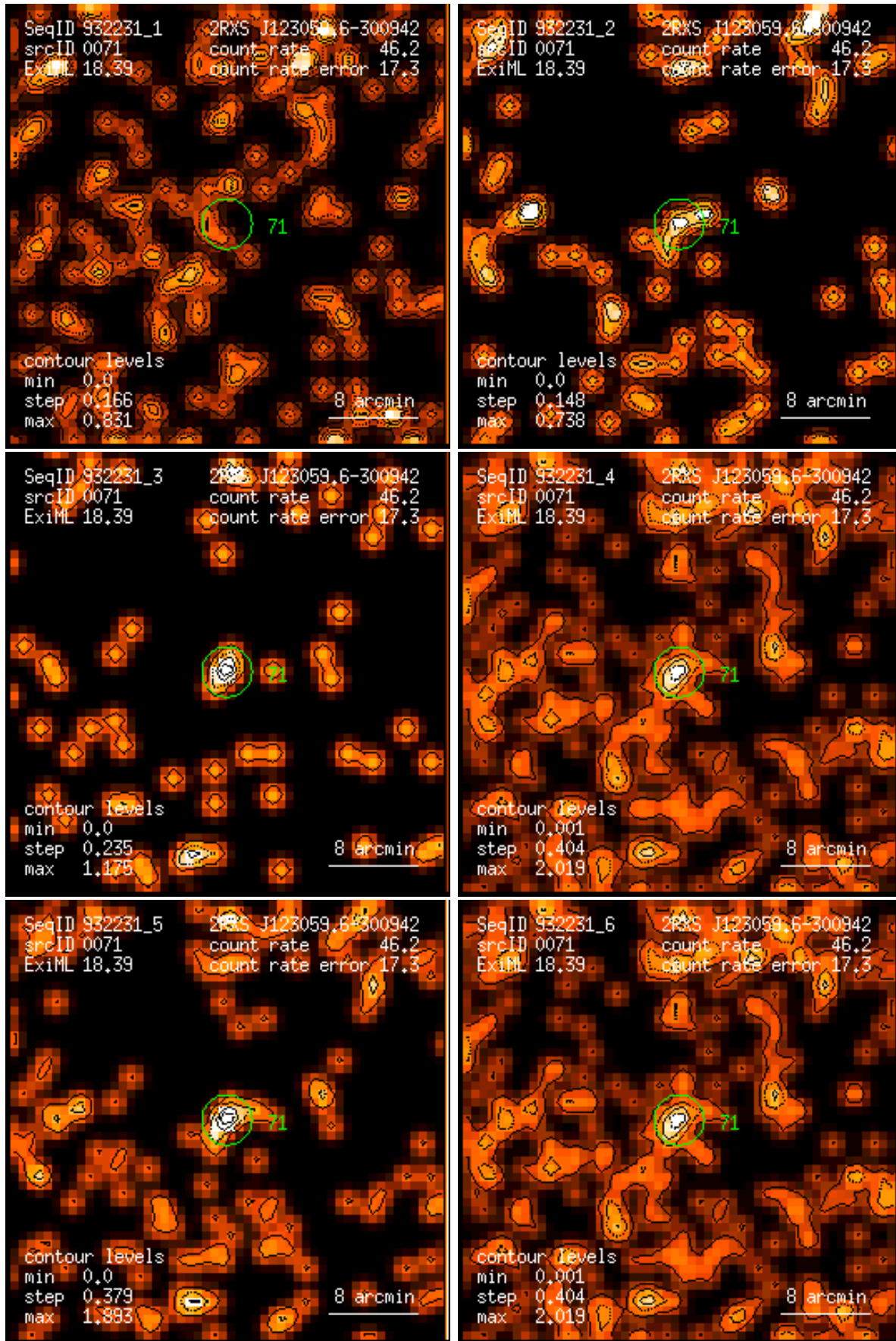
Figure 71: RASS 932231: detection 0071: band rate images, Gaussian filter: (1) PSPC channels 11 – 41, (2) 52 – 90, (3) 91 – 201, (4) 11 – 235, (5) 52 – 201, (6) 11 – 201. Broad band rates in counts/ks. Band rate contour levels in counts/ks/arcmin 2 .
