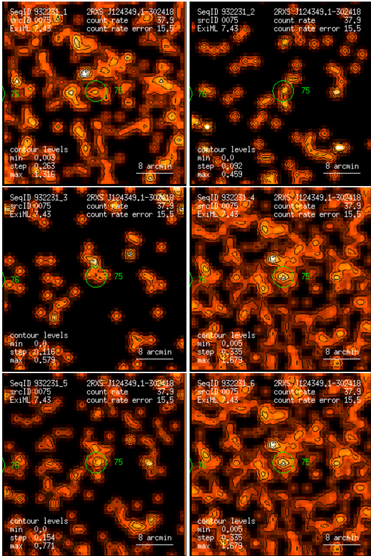
Figure 75: RASS 932231: detection 0075: band rate images, Gaussian filter: (1) PSPC channels 11 – 41, (2) 52 – 90, (3) 91 – 201, (4) 11 – 235, (5) 52 – 201, (6) 11 – 201. Broad band rates in counts/ks. Band rate contour levels in counts/ks/arcmin 2 .
