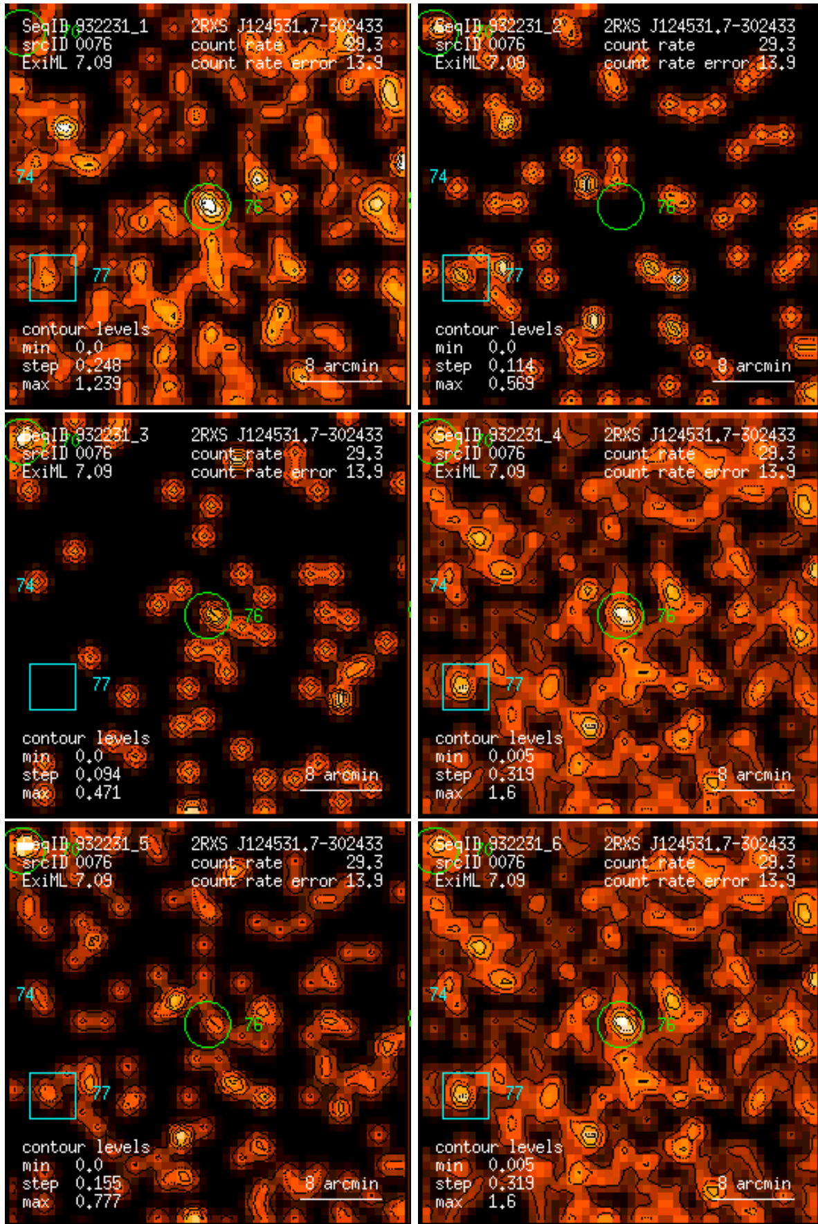
Figure 76: RASS 932231: detection 0076: band rate images, Gaussian filter: (1) PSPC channels 11 – 41, (2) 52 – 90, (3) 91 – 201, (4) 11 – 235, (5) 52 – 201, (6) 11 – 201. Broad band rates in counts/ks. Band rate contour levels in counts/ks/arcmin 2 .
