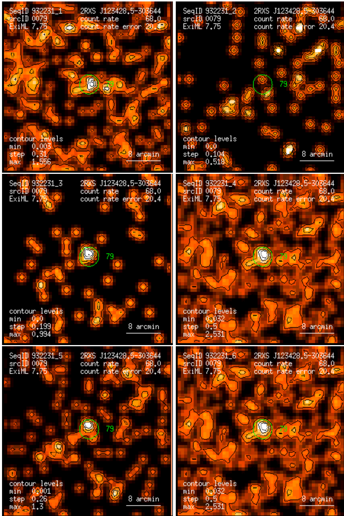
Figure 79: RASS 932231: detection 0079: band rate images, Gaussian filter: (1) PSPC channels 11 – 41, (2) 52 – 90, (3) 91 – 201, (4) 11 – 235, (5) 52 – 201, (6) 11 – 201. Broad band rates in counts/ks. Band rate contour levels in counts/ks/arcmin 2 .
