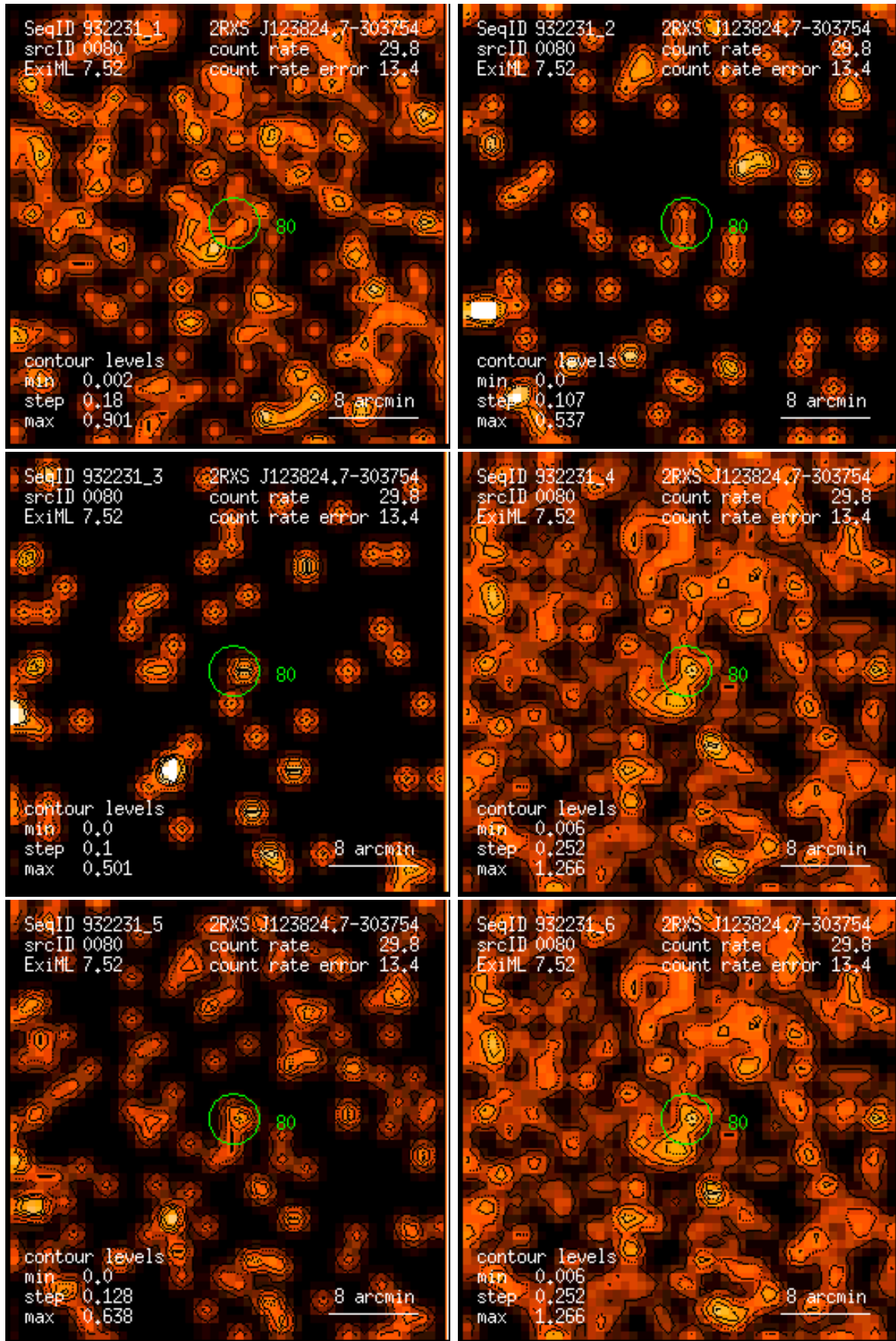
Figure 80: RASS 932231: detection 0080: band rate images, Gaussian filter: (1) PSPC channels 11 – 41, (2) 52 – 90, (3) 91 – 201, (4) 11 – 235, (5) 52 – 201, (6) 11 – 201. Broad band rates in counts/ks. Band rate contour levels in counts/ks/arcmin 2 .
