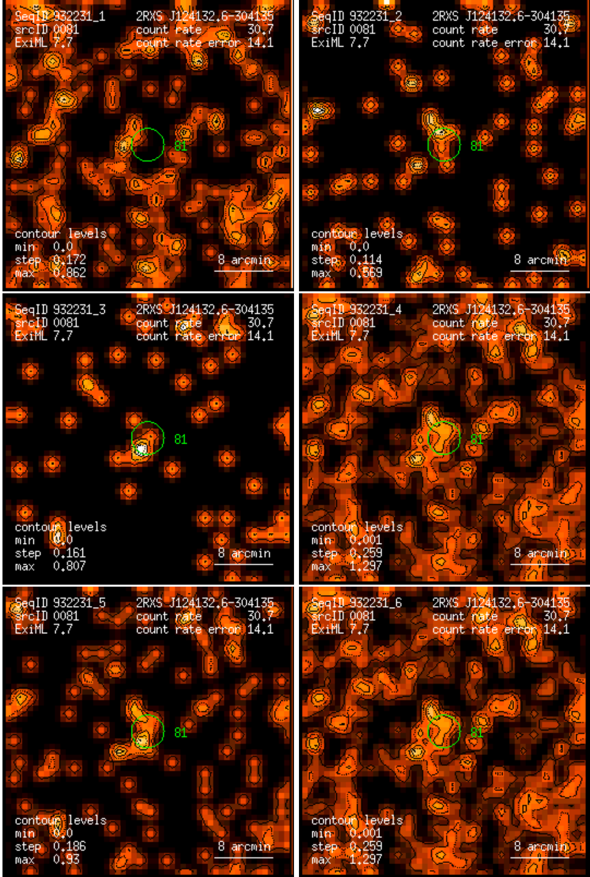
Figure 81: RASS 932231: detection 0081: band rate images, Gaussian filter: (1) PSPC channels 11 – 41, (2) 52 – 90, (3) 91 – 201, (4) 11 – 235, (5) 52 – 201, (6) 11 – 201. Broad band rates in counts/ks. Band rate contour levels in counts/ks/arcmin 2 .
