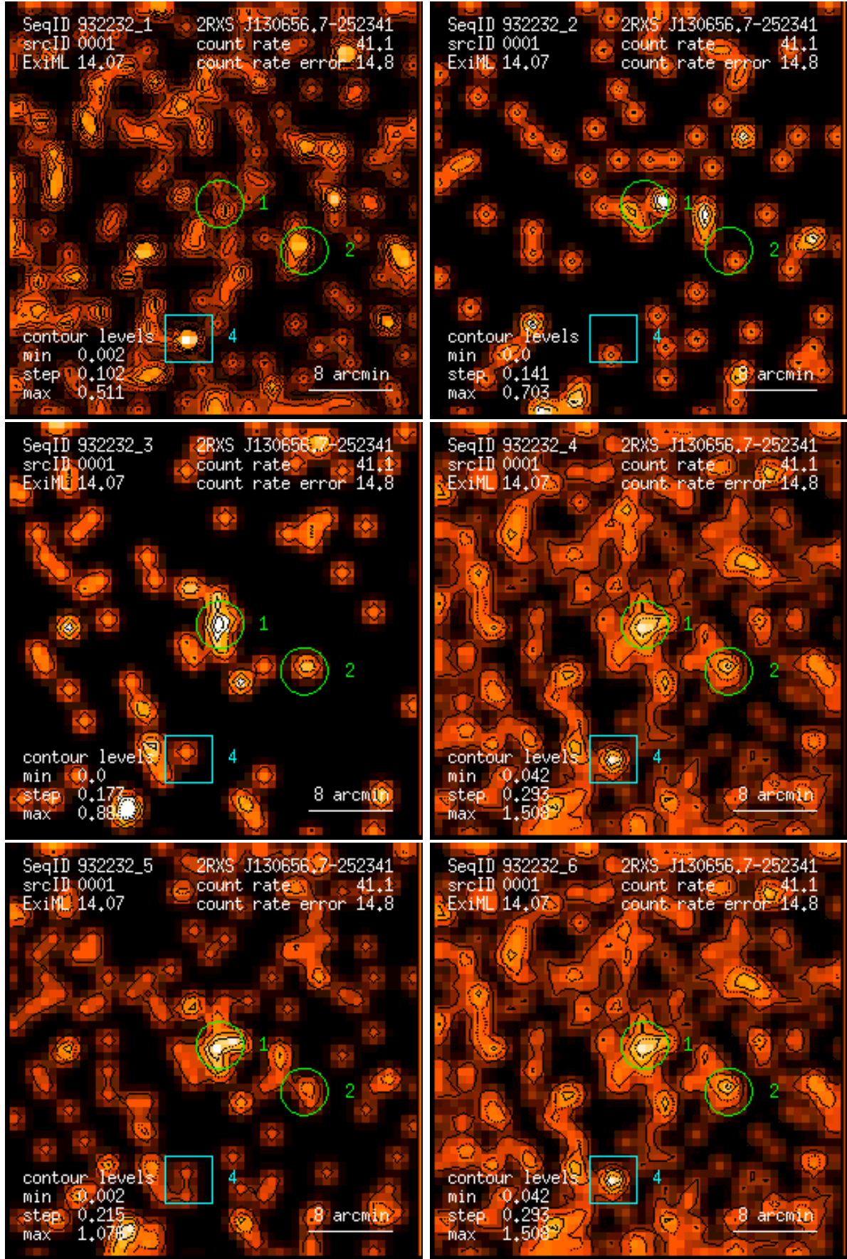
Figure 1: RASS 932232: detection 0001: band rate images, Gaussian filter: (1) PSPC channels 11 – 41, (2) 52 – 90, (3) 91 – 201, (4) 11 – 235, (5) 52 – 201, (6) 11 – 201. Broad band rates in counts/ks. Band rate contour levels in counts/ks/arcmin 2 .
