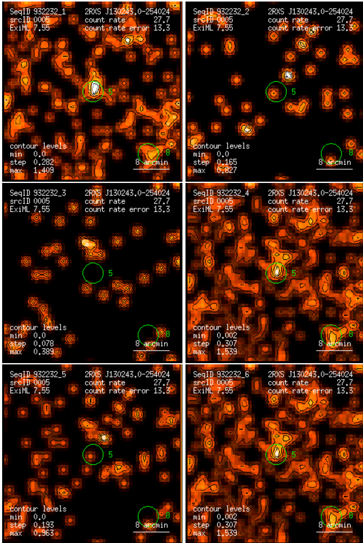
Figure 5: RASS 932232: detection 0005: band rate images, Gaussian filter: (1) PSPC channels 11 – 41, (2) 52 – 90, (3) 91 – 201, (4) 11 – 235, (5) 52 – 201, (6) 11 – 201. Broad band rates in counts/ks. Band rate contour levels in counts/ks/arcmin 2 .
