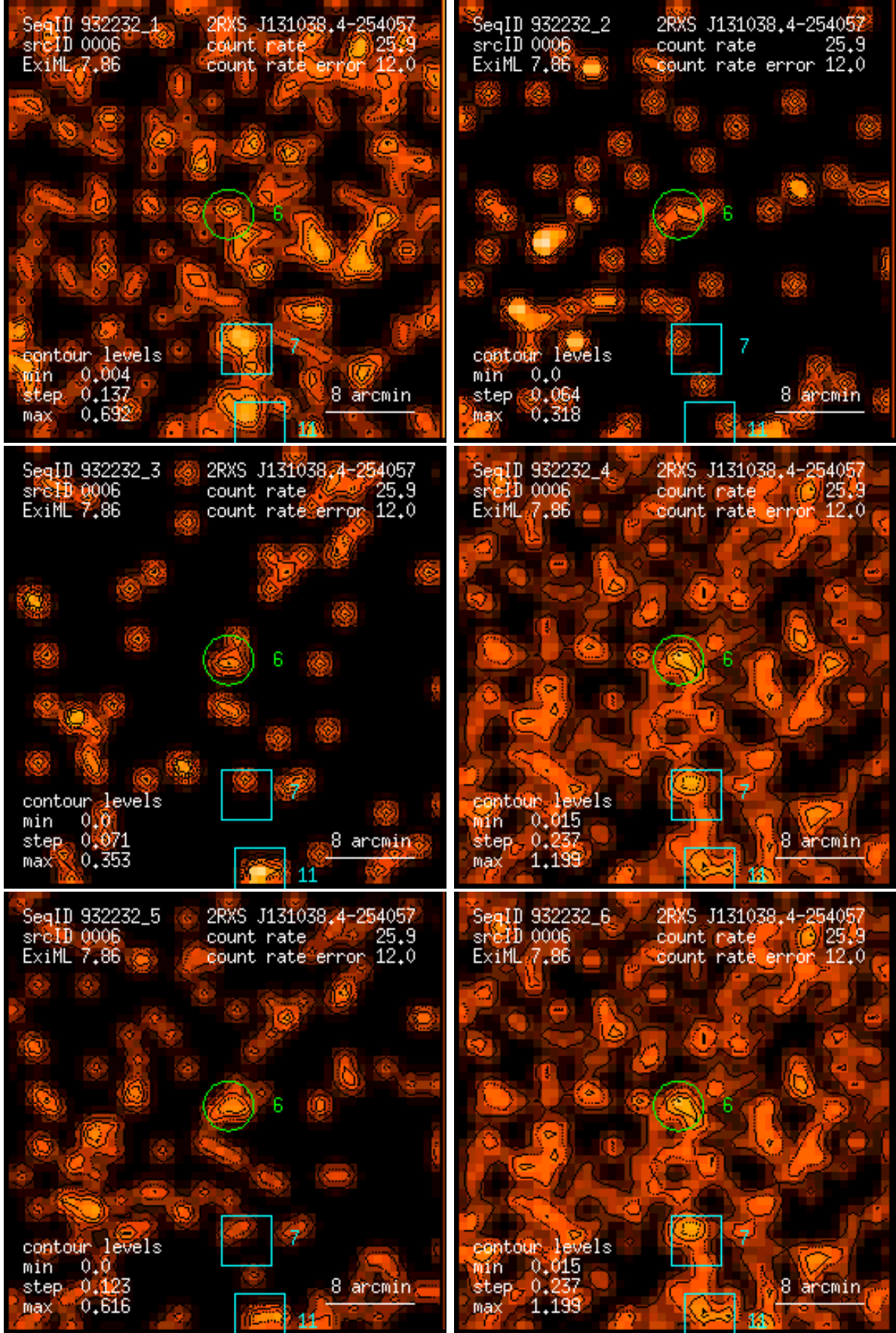
Figure 6: RASS 932232: detection 0006: band rate images, Gaussian filter: (1) PSPC channels 11 – 41, (2) 52 – 90, (3) 91 – 201, (4) 11 – 235, (5) 52 – 201, (6) 11 – 201. Broad band rates in counts/ks. Band rate contour levels in counts/ks/arcmin 2 .
