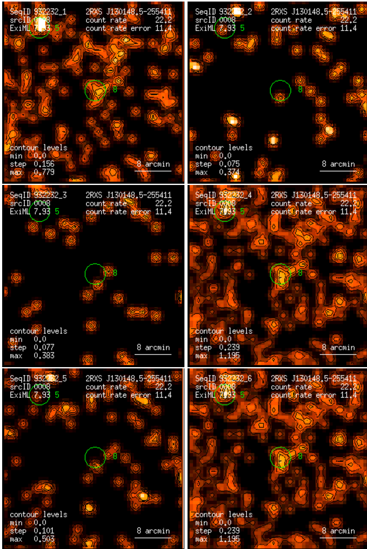
Figure 8: RASS 932232: detection 0008: band rate images, Gaussian filter: (1) PSPC channels 11 – 41, (2) 52 – 90, (3) 91 – 201, (4) 11 – 235, (5) 52 – 201, (6) 11 – 201. Broad band rates in counts/ks. Band rate contour levels in counts/ks/arcmin 2 .
