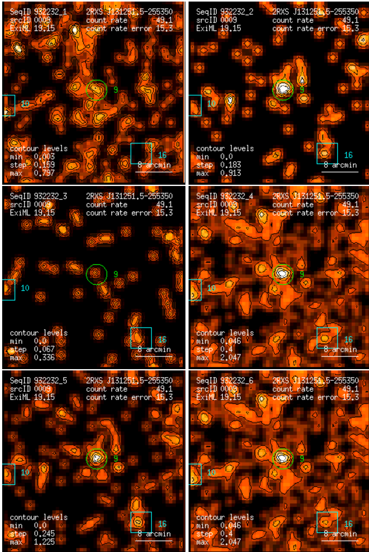
Figure 9: RASS 932232: detection 0009: band rate images, Gaussian filter: (1) PSPC channels 11 – 41, (2) 52 – 90, (3) 91 – 201, (4) 11 – 235, (5) 52 – 201, (6) 11 – 201. Broad band rates in counts/ks. Band rate contour levels in counts/ks/arcmin 2 .
