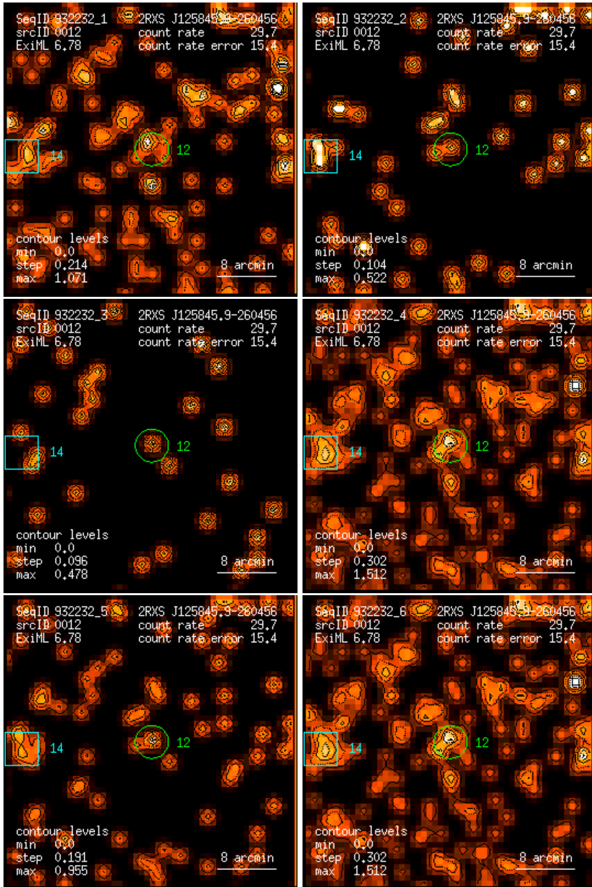
Figure 12: RASS 932232: detection 0012: band rate images, Gaussian filter: (1) PSPC channels 11 – 41, (2) 52 – 90, (3) 91 – 201, (4) 11 – 235, (5) 52 – 201, (6) 11 – 201. Broad band rates in counts/ks. Band rate contour levels in counts/ks/arcmin 2 .
