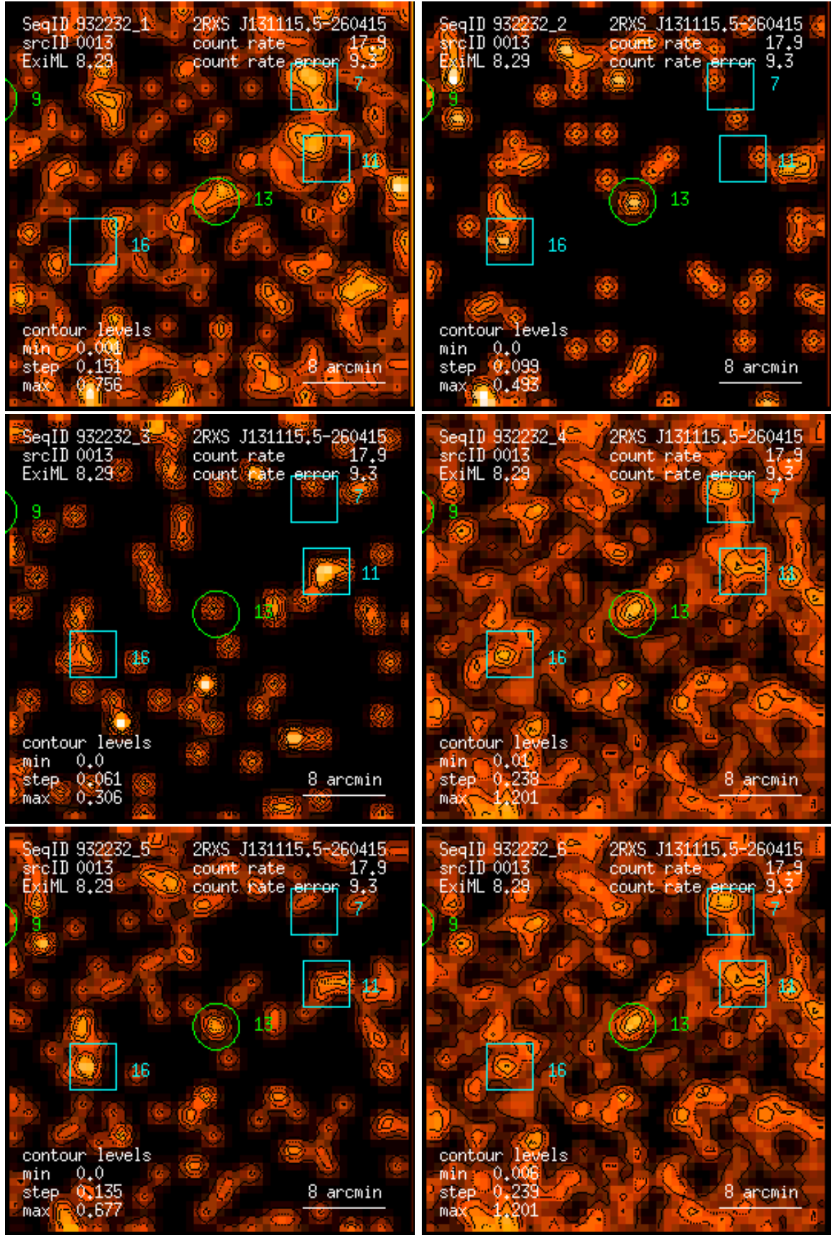
Figure 13: RASS 932232: detection 0013: band rate images, Gaussian filter: (1) PSPC channels 11 – 41, (2) 52 – 90, (3) 91 – 201, (4) 11 – 235, (5) 52 – 201, (6) 11 – 201. Broad band rates in counts/ks. Band rate contour levels in counts/ks/arcmin 2 .
