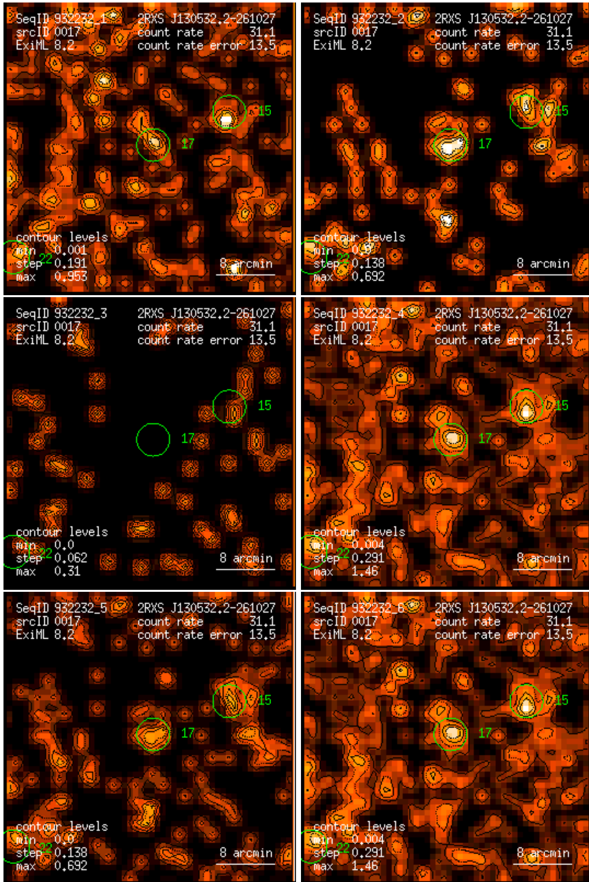
Figure 17: RASS 932232: detection 0017: band rate images, Gaussian filter: (1) PSPC channels 11 – 41, (2) 52 – 90, (3) 91 – 201, (4) 11 – 235, (5) 52 – 201, (6) 11 – 201. Broad band rates in counts/ks. Band rate contour levels in counts/ks/arcmin 2 .
