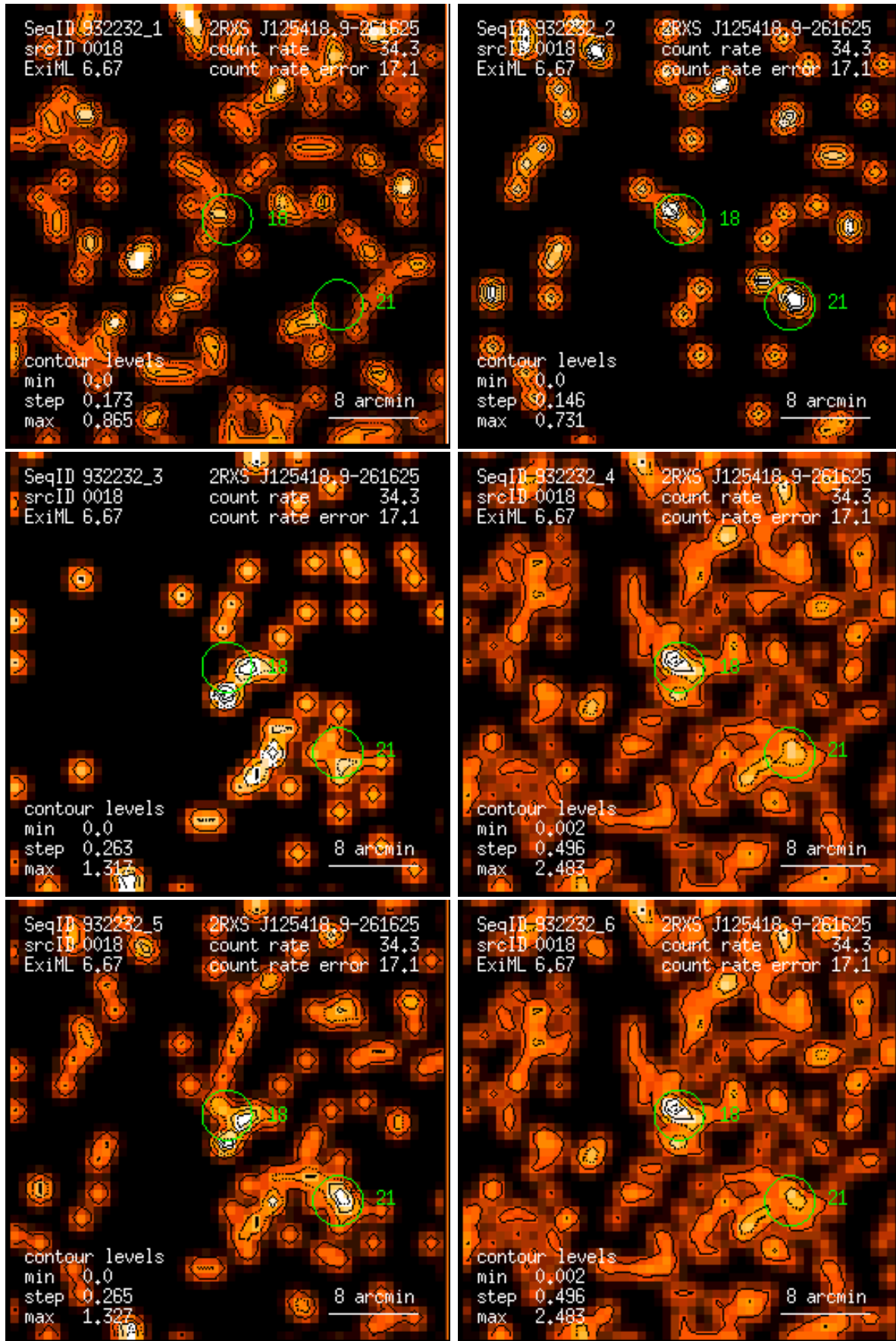
Figure 18: RASS 932232: detection 0018: band rate images, Gaussian filter: (1) PSPC channels 11 – 41, (2) 52 – 90, (3) 91 – 201, (4) 11 – 235, (5) 52 – 201, (6) 11 – 201. Broad band rates in counts/ks. Band rate contour levels in counts/ks/arcmin 2 .
