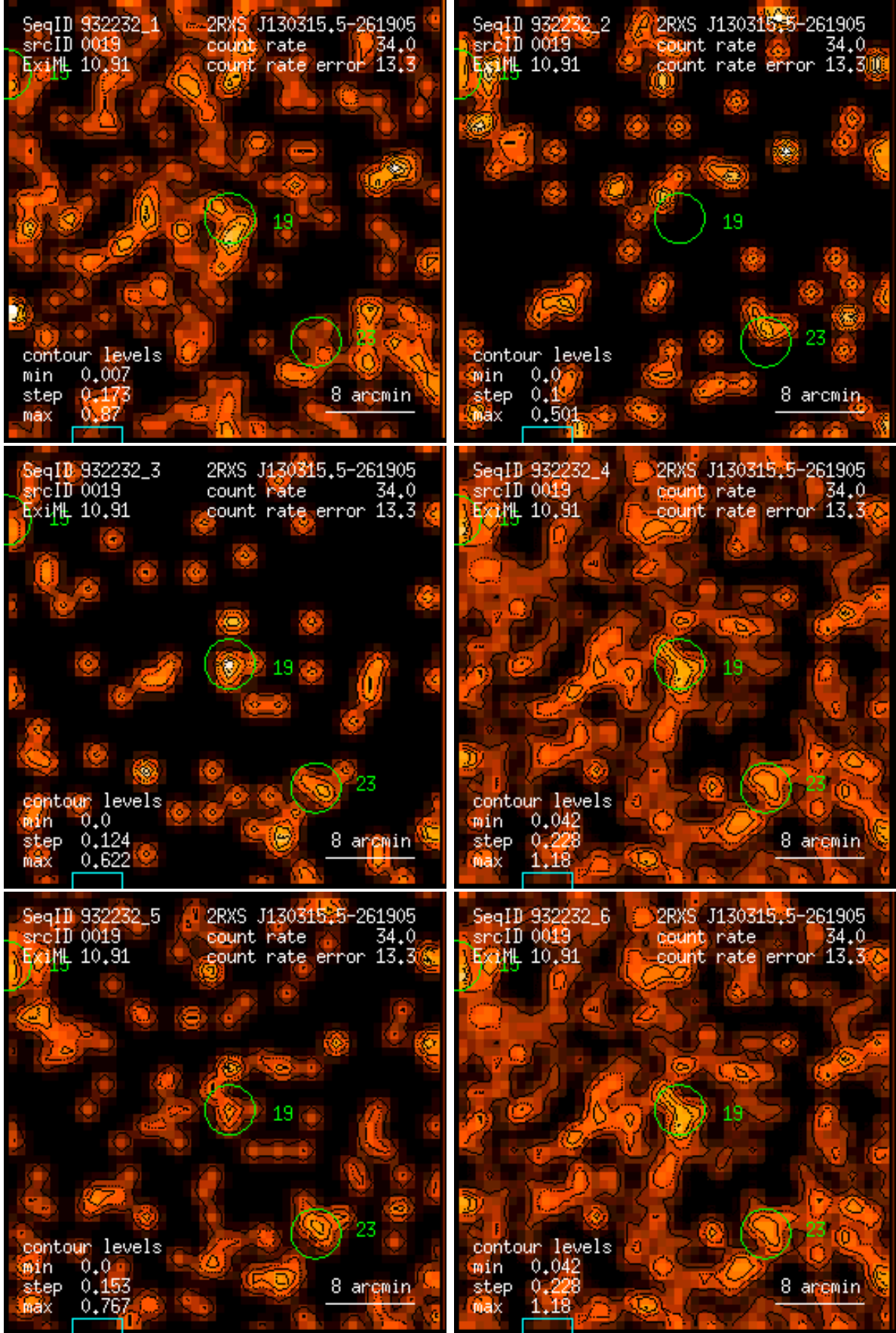
Figure 19: RASS 932232: detection 0019: band rate images, Gaussian filter: (1) PSPC channels 11 – 41, (2) 52 – 90, (3) 91 – 201, (4) 11 – 235, (5) 52 – 201, (6) 11 – 201. Broad band rates in counts/ks. Band rate contour levels in counts/ks/arcmin 2 .
