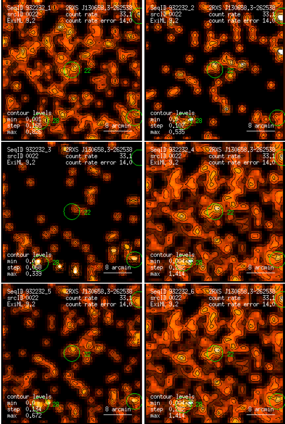
Figure 22: RASS 932232: detection 0022: band rate images, Gaussian filter: (1) PSPC channels 11 – 41, (2) 52 – 90, (3) 91 – 201, (4) 11 – 235, (5) 52 – 201, (6) 11 – 201. Broad band rates in counts/ks. Band rate contour levels in counts/ks/arcmin 2 .
