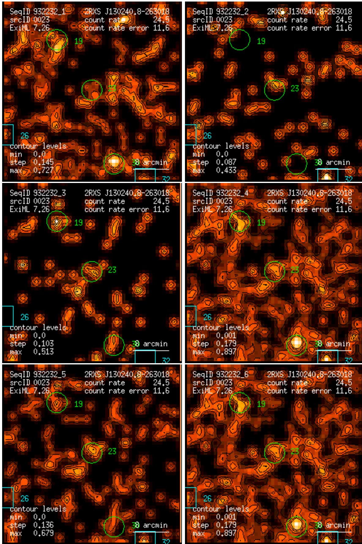
Figure 23: RASS 932232: detection 0023: band rate images, Gaussian filter: (1) PSPC channels 11 – 41, (2) 52 – 90, (3) 91 – 201, (4) 11 – 235, (5) 52 – 201, (6) 11 – 201. Broad band rates in counts/ks. Band rate contour levels in counts/ks/arcmin 2 .
