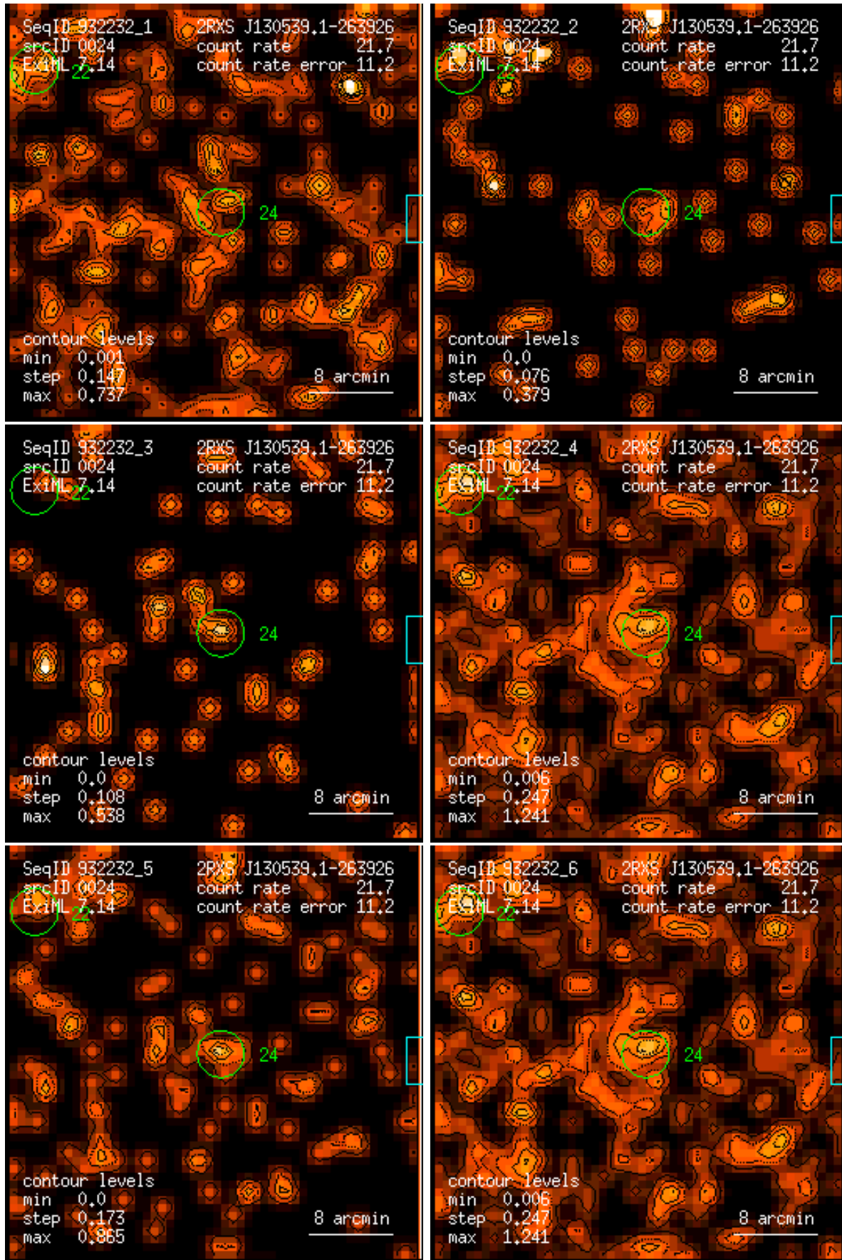
Figure 24: RASS 932232: detection 0024: band rate images, Gaussian filter: (1) PSPC channels 11 – 41, (2) 52 – 90, (3) 91 – 201, (4) 11 – 235, (5) 52 – 201, (6) 11 – 201. Broad band rates in counts/ks. Band rate contour levels in counts/ks/arcmin 2 .
