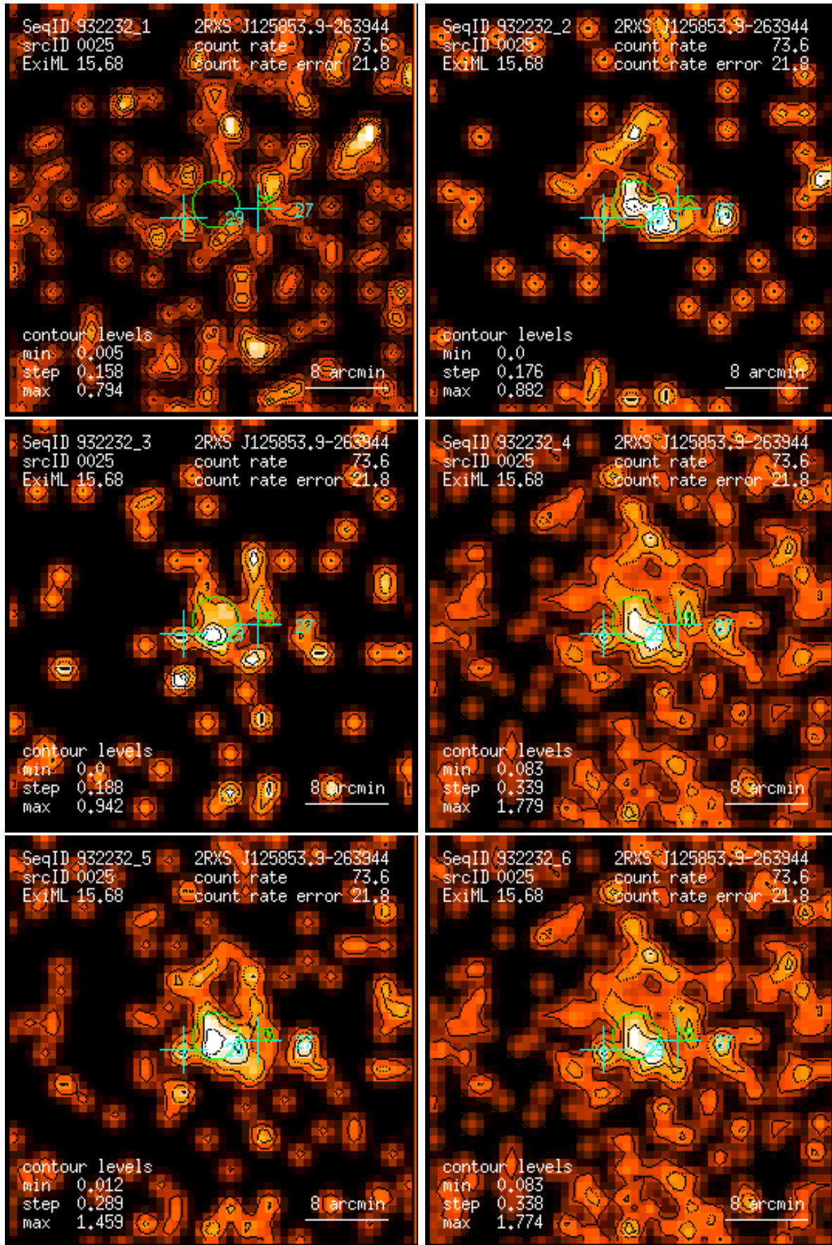
Figure 25: RASS 932232: detection 0025: band rate images, Gaussian filter: (1) PSPC channels 11 – 41, (2) 52 – 90, (3) 91 – 201, (4) 11 – 235, (5) 52 – 201, (6) 11 – 201. Broad band rates in counts/ks. Band rate contour levels in counts/ks/arcmin 2 .
