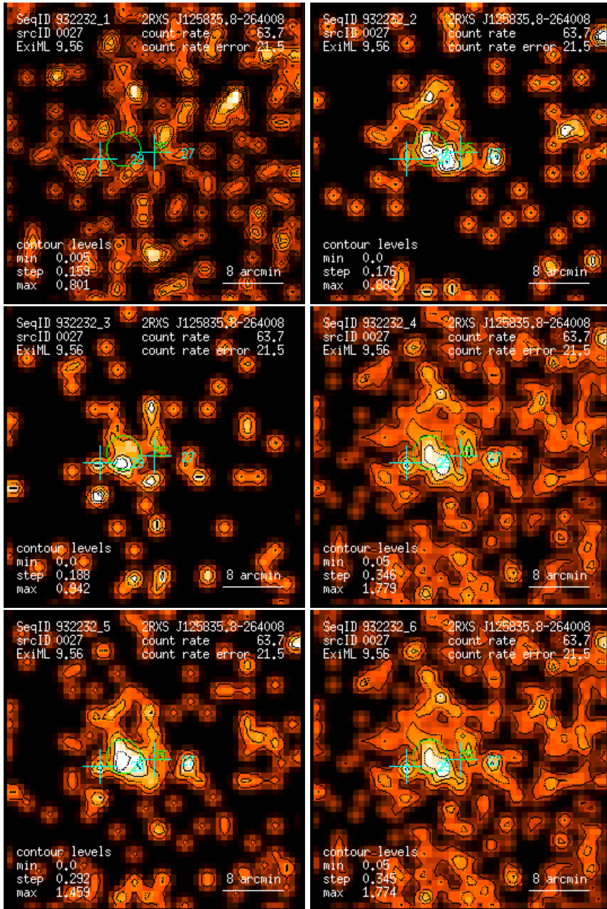
Figure 27: RASS 932232: detection 0027: band rate images, Gaussian filter: (1) PSPC channels 11 – 41, (2) 52 – 90, (3) 91 – 201, (4) 11 – 235, (5) 52 – 201, (6) 11 – 201. Broad band rates in counts/ks. Band rate contour levels in counts/ks/arcmin 2 .
