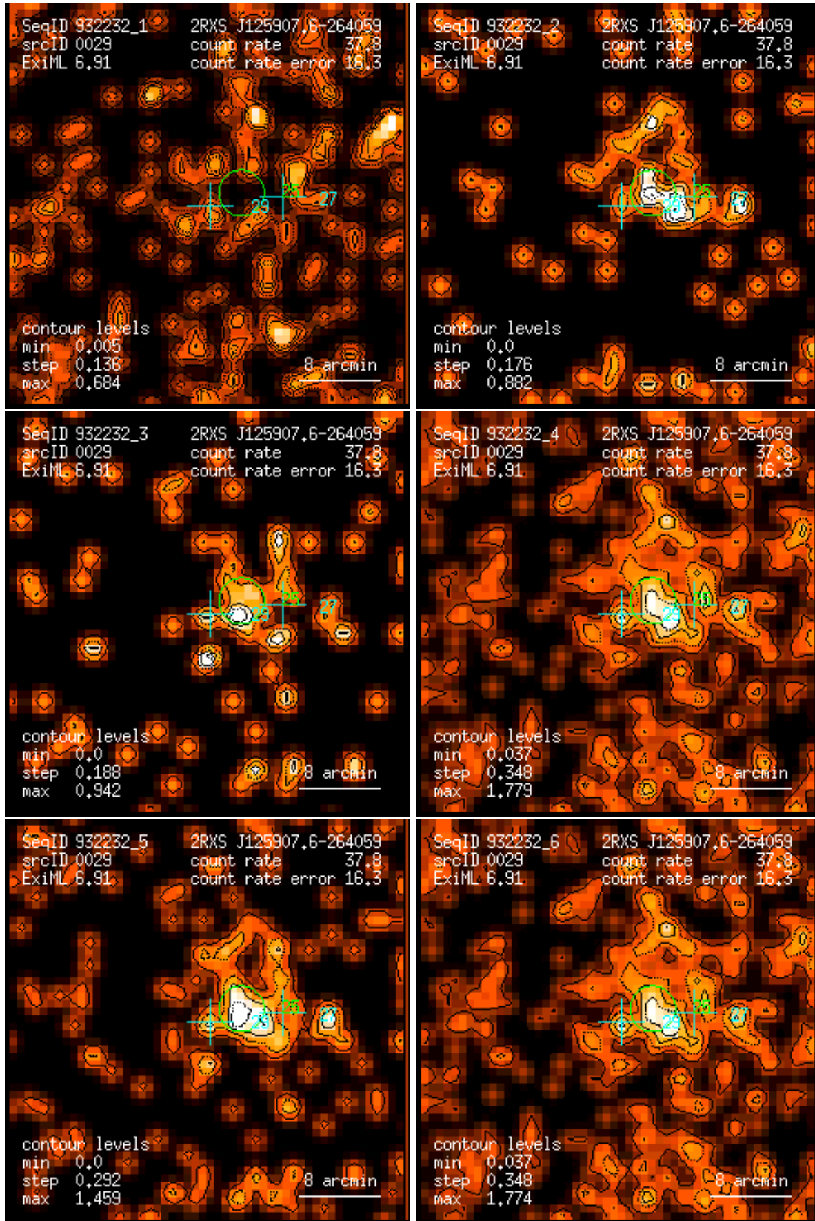
Figure 29: RASS 932232: detection 0029: band rate images, Gaussian filter: (1) PSPC channels 11 – 41, (2) 52 – 90, (3) 91 – 201, (4) 11 – 235, (5) 52 – 201, (6) 11 – 201. Broad band rates in counts/ks. Band rate contour levels in counts/ks/arcmin 2 .
