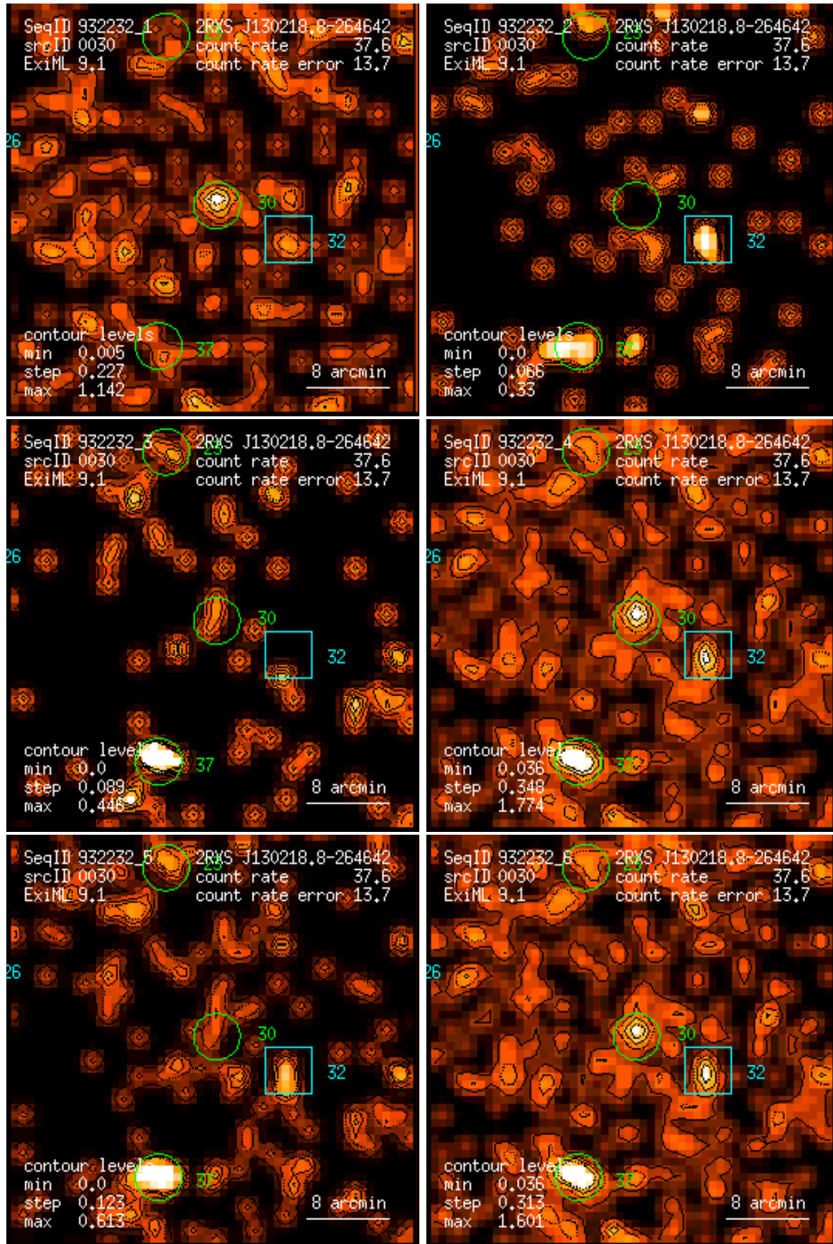
Figure 30: RASS 932232: detection 0030: band rate images, Gaussian filter: (1) PSPC channels 11 – 41, (2) 52 – 90, (3) 91 – 201, (4) 11 – 235, (5) 52 – 201, (6) 11 – 201. Broad band rates in counts/ks. Band rate contour levels in counts/ks/arcmin 2 .
