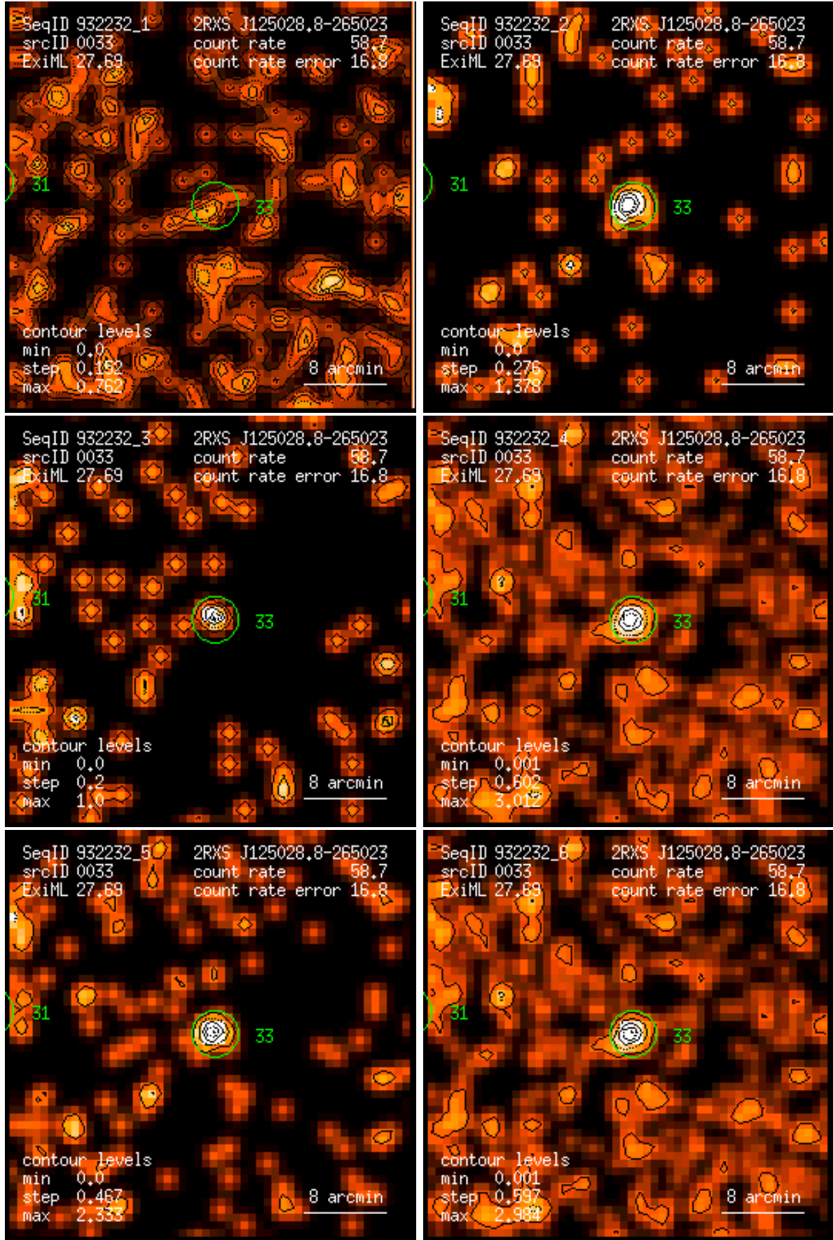
Figure 33: RASS 932232: detection 0033: band rate images, Gaussian filter: (1) PSPC channels 11 – 41, (2) 52 – 90, (3) 91 – 201, (4) 11 – 235, (5) 52 – 201, (6) 11 – 201. Broad band rates in counts/ks. Band rate contour levels in counts/ks/arcmin 2 .
