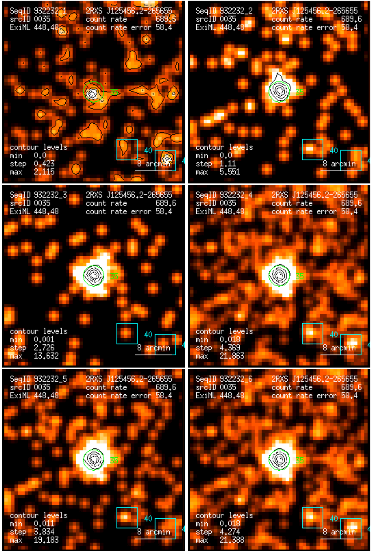
Figure 35: RASS 932232: detection 0035: band rate images, Gaussian filter: (1) PSPC channels 11 – 41, (2) 52 – 90, (3) 91 – 201, (4) 11 – 235, (5) 52 – 201, (6) 11 – 201. Broad band rates in counts/ks. Band rate contour levels in counts/ks/arcmin 2 .
