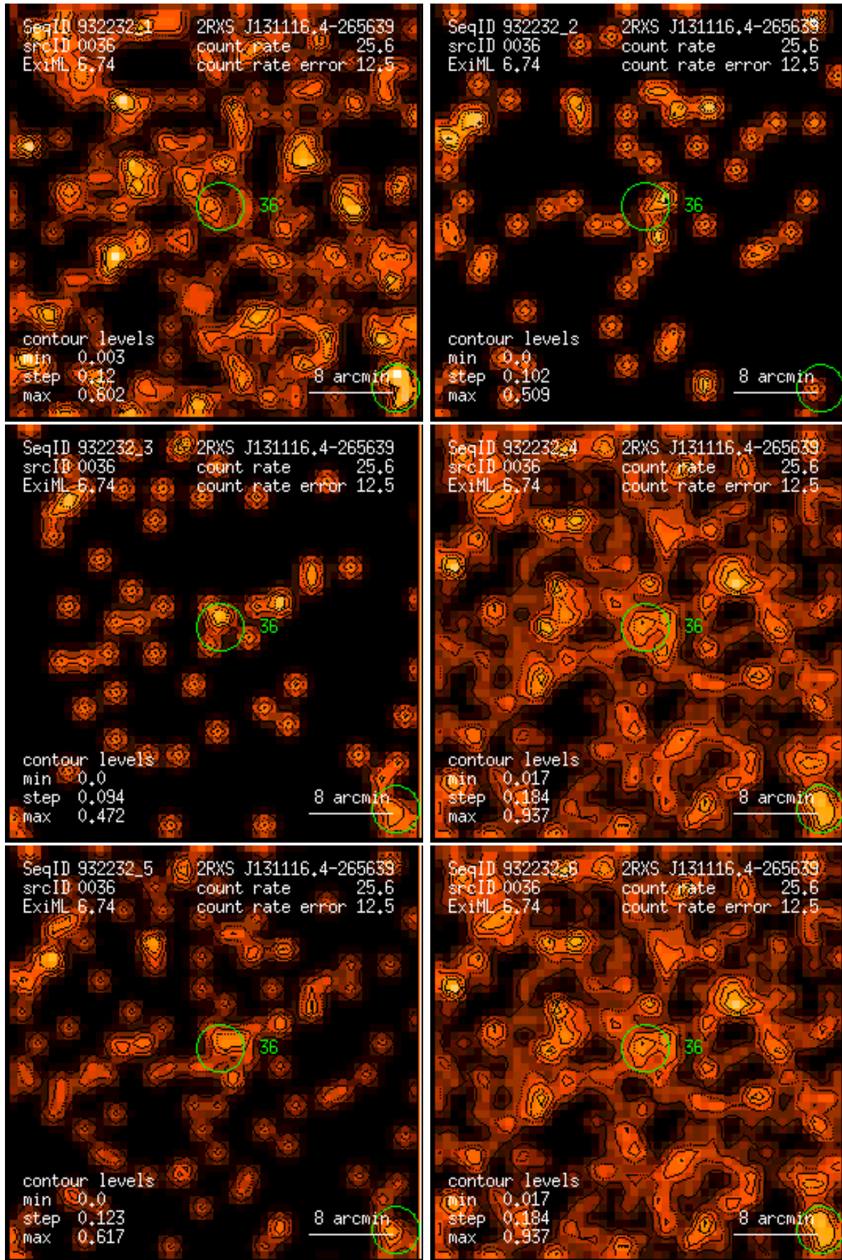
Figure 36: RASS 932232: detection 0036: band rate images, Gaussian filter: (1) PSPC channels 11 – 41, (2) 52 – 90, (3) 91 – 201, (4) 11 – 235, (5) 52 – 201, (6) 11 – 201. Broad band rates in counts/ks. Band rate contour levels in counts/ks/arcmin 2 .
