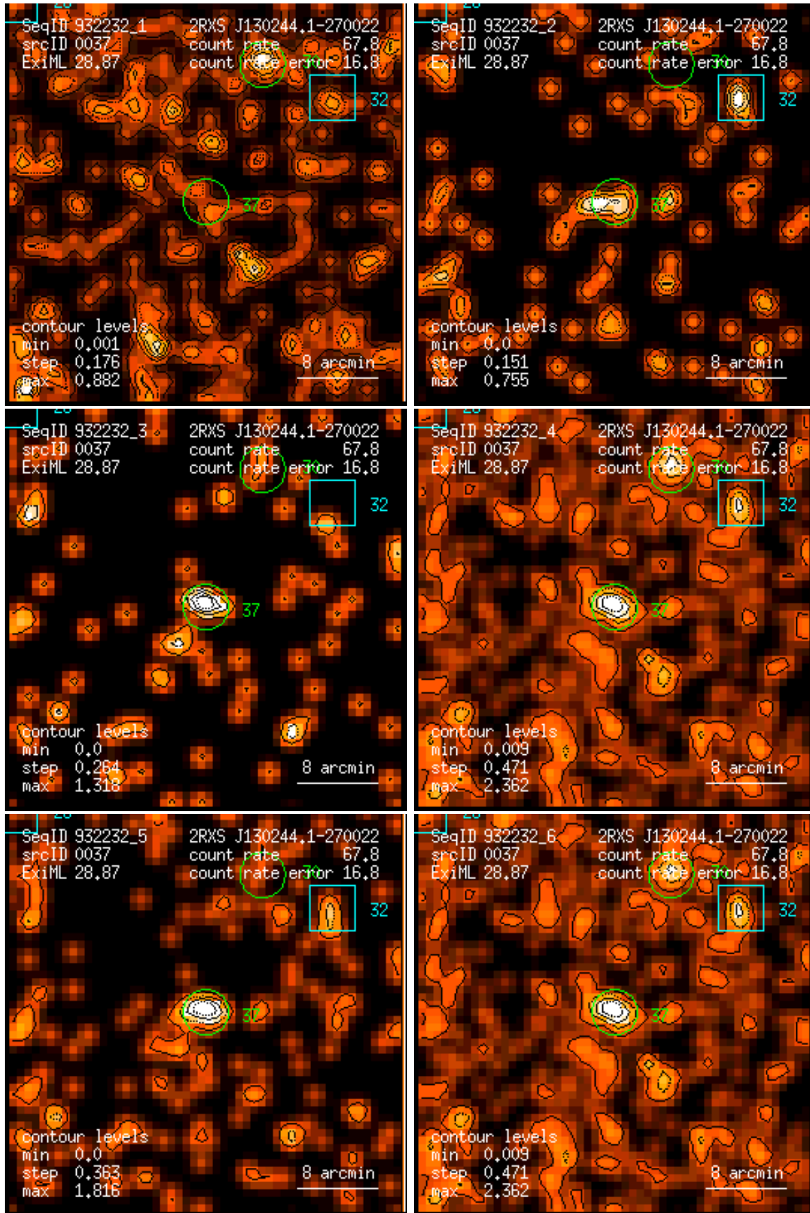
Figure 37: RASS 932232: detection 0037: band rate images, Gaussian filter: (1) PSPC channels 11 – 41, (2) 52 – 90, (3) 91 – 201, (4) 11 – 235, (5) 52 – 201, (6) 11 – 201. Broad band rates in counts/ks. Band rate contour levels in counts/ks/arcmin 2 .
