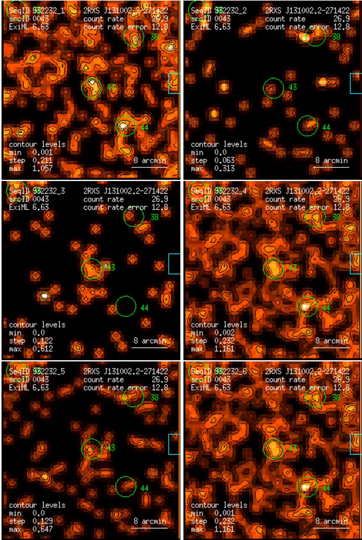
Figure 43: RASS 932232: detection 0043: band rate images, Gaussian filter: (1) PSPC channels 11 – 41, (2) 52 – 90, (3) 91 – 201, (4) 11 – 235, (5) 52 – 201, (6) 11 – 201. Broad band rates in counts/ks. Band rate contour levels in counts/ks/arcmin 2 .
