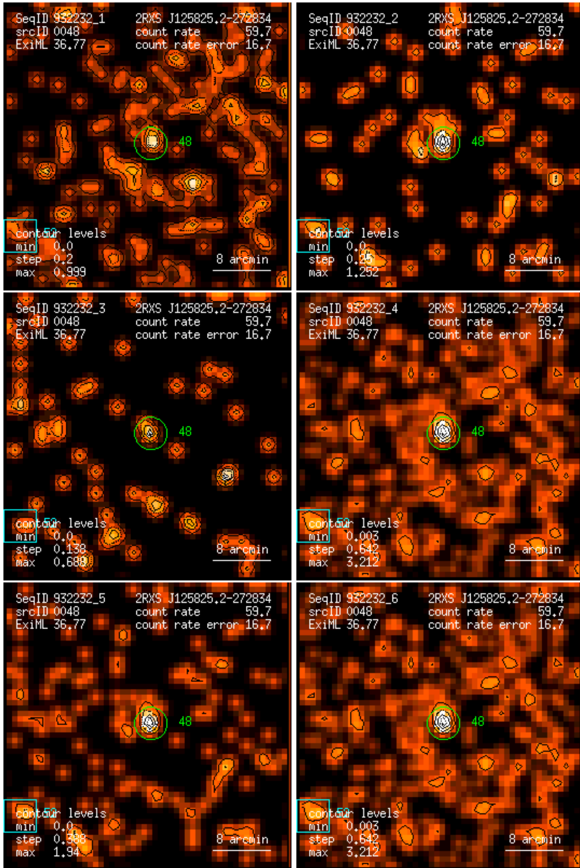
Figure 48: RASS 932232: detection 0048: band rate images, Gaussian filter: (1) PSPC channels 11 – 41, (2) 52 – 90, (3) 91 – 201, (4) 11 – 235, (5) 52 – 201, (6) 11 – 201. Broad band rates in counts/ks. Band rate contour levels in counts/ks/arcmin 2 .
