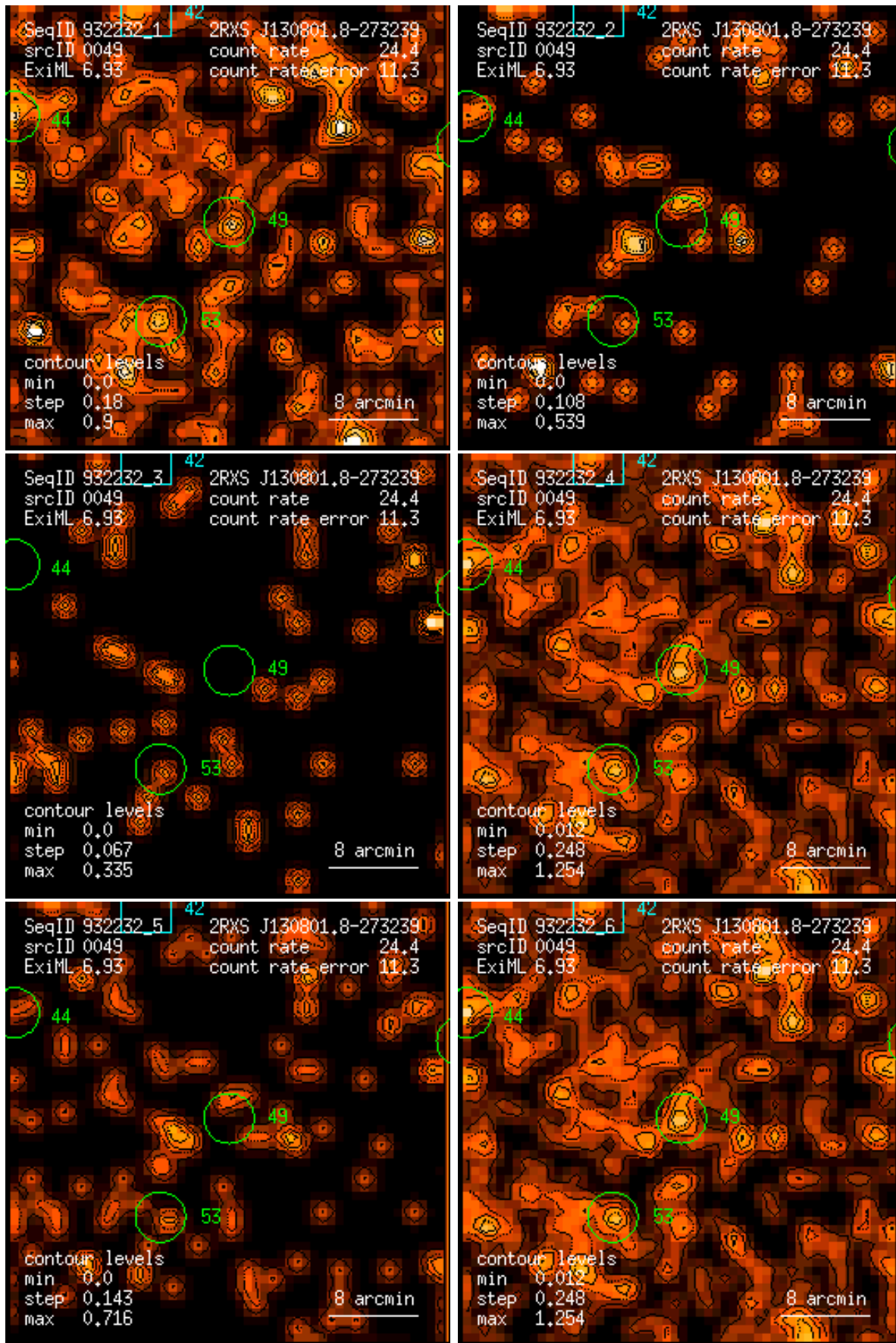
Figure 49: RASS 932232: detection 0049: band rate images, Gaussian filter: (1) PSPC channels 11 – 41, (2) 52 – 90, (3) 91 – 201, (4) 11 – 235, (5) 52 – 201, (6) 11 – 201. Broad band rates in counts/ks. Band rate contour levels in counts/ks/arcmin 2 .
