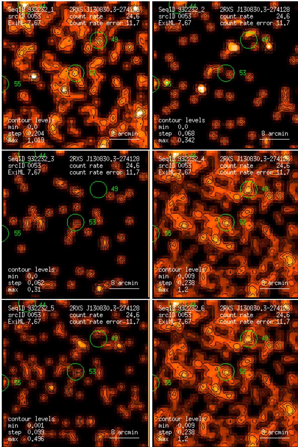
Figure 53: RASS 932232: detection 0053: band rate images, Gaussian filter: (1) PSPC channels 11 – 41, (2) 52 – 90, (3) 91 – 201, (4) 11 – 235, (5) 52 – 201, (6) 11 – 201. Broad band rates in counts/ks. Band rate contour levels in counts/ks/arcmin 2 .
