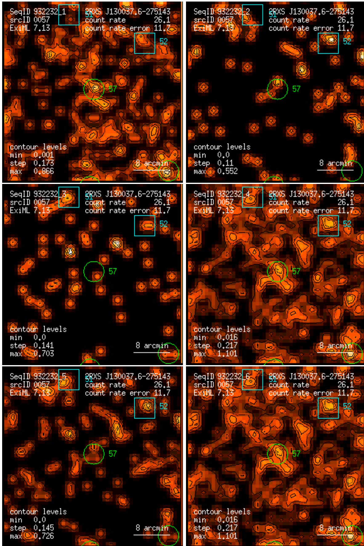
Figure 57: RASS 932232: detection 0057: band rate images, Gaussian filter: (1) PSPC channels 11 – 41, (2) 52 – 90, (3) 91 – 201, (4) 11 – 235, (5) 52 – 201, (6) 11 – 201. Broad band rates in counts/ks. Band rate contour levels in counts/ks/arcmin 2 .
