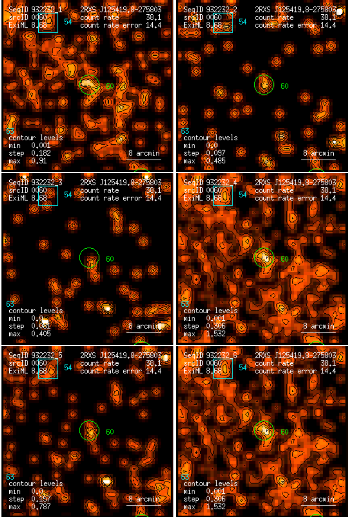
Figure 60: RASS 932232: detection 0060: band rate images, Gaussian filter: (1) PSPC channels 11 – 41, (2) 52 – 90, (3) 91 – 201, (4) 11 – 235, (5) 52 – 201, (6) 11 – 201. Broad band rates in counts/ks. Band rate contour levels in counts/ks/arcmin 2 .
