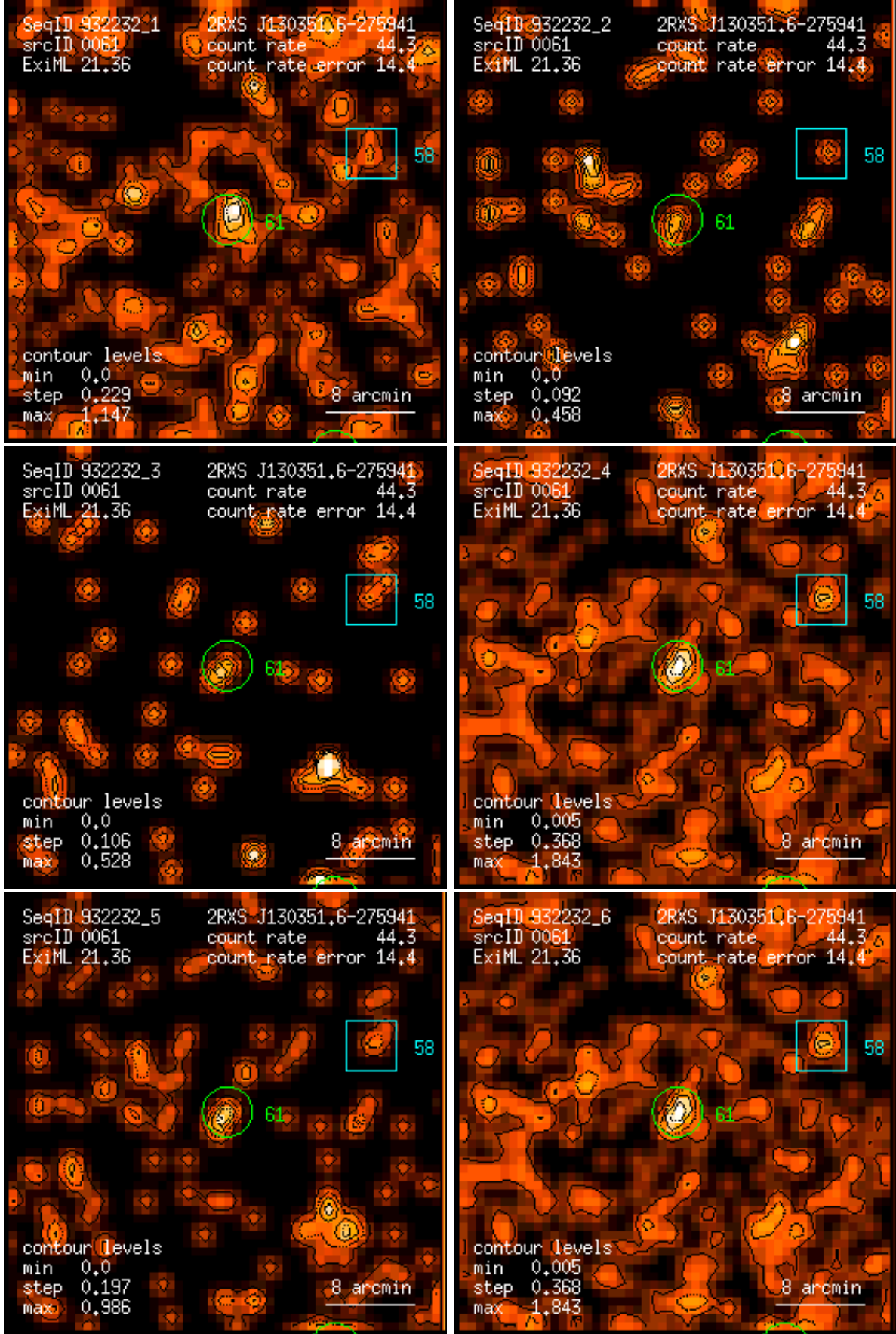
Figure 61: RASS 932232: detection 0061: band rate images, Gaussian filter: (1) PSPC channels 11 – 41, (2) 52 – 90, (3) 91 – 201, (4) 11 – 235, (5) 52 – 201, (6) 11 – 201. Broad band rates in counts/ks. Band rate contour levels in counts/ks/arcmin 2 .
