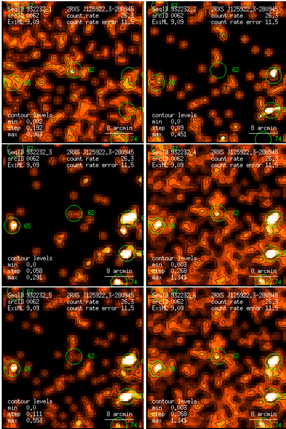
Figure 62: RASS 932232: detection 0062: band rate images, Gaussian filter: (1) PSPC channels 11 – 41, (2) 52 – 90, (3) 91 – 201, (4) 11 – 235, (5) 52 – 201, (6) 11 – 201. Broad band rates in counts/ks. Band rate contour levels in counts/ks/arcmin 2 .
