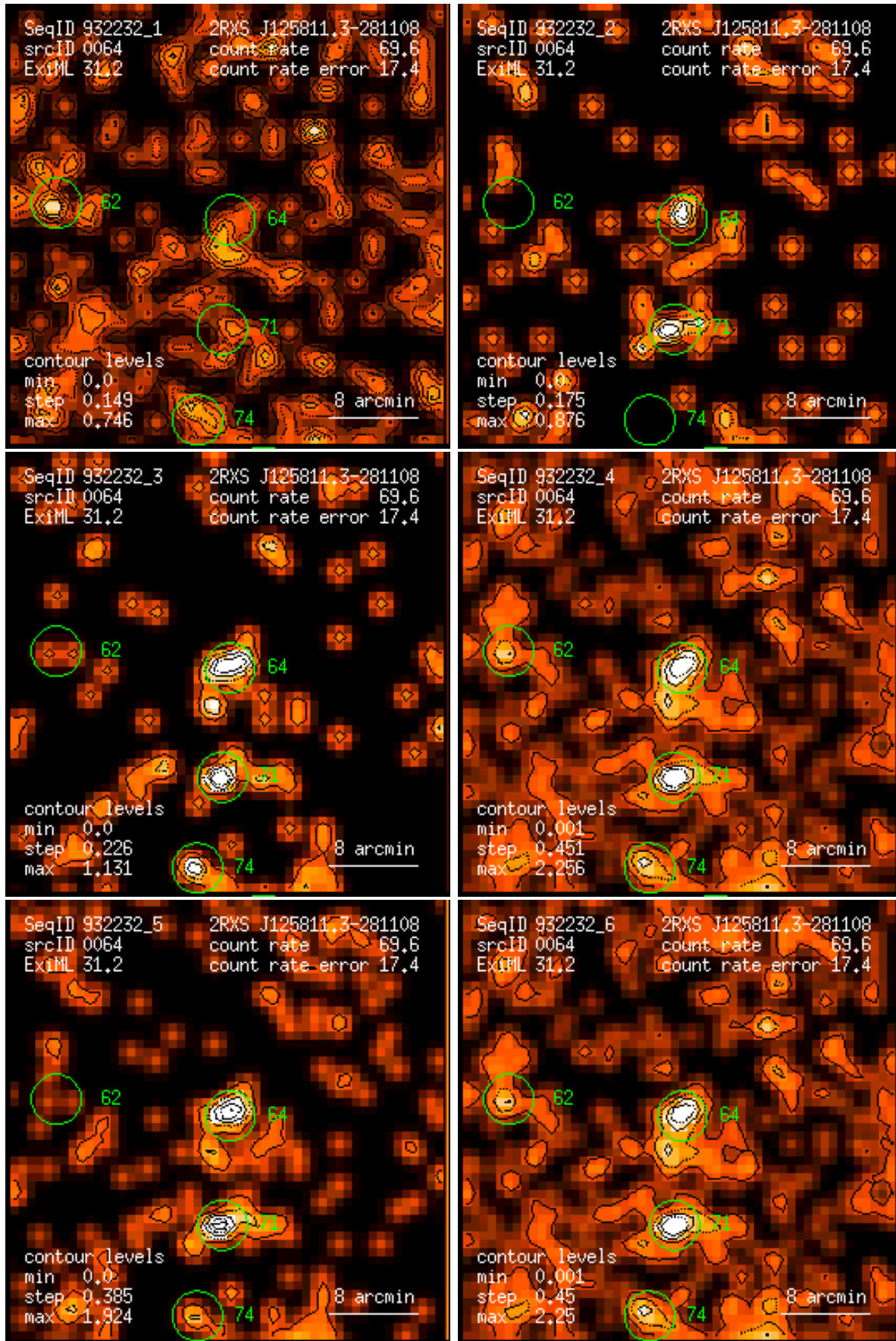
Figure 64: RASS 932232: detection 0064: band rate images, Gaussian filter: (1) PSPC channels 11 – 41, (2) 52 – 90, (3) 91 – 201, (4) 11 – 235, (5) 52 – 201, (6) 11 – 201. Broad band rates in counts/ks. Band rate contour levels in counts/ks/arcmin 2 .
