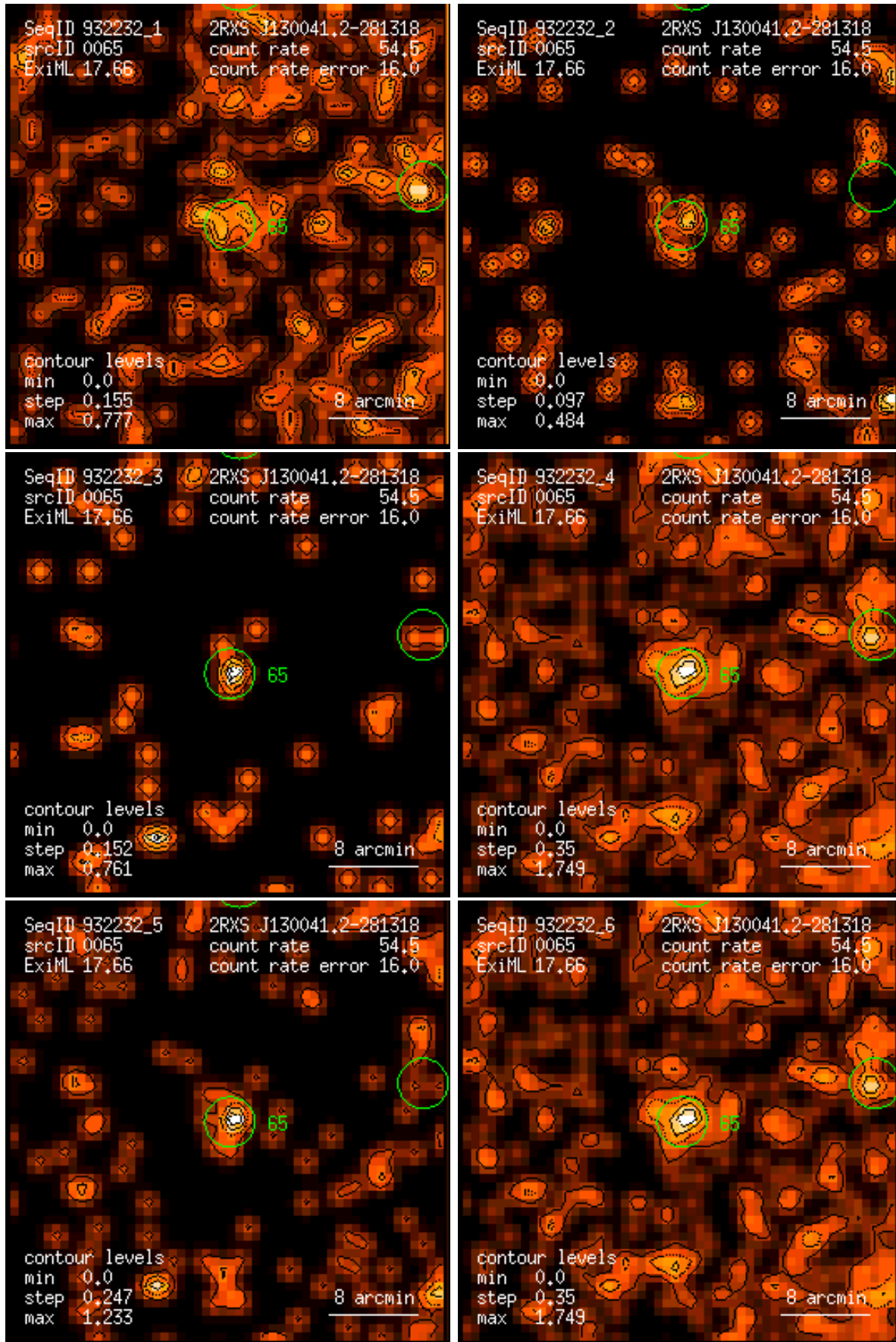
Figure 65: RASS 932232: detection 0065: band rate images, Gaussian filter: (1) PSPC channels 11 – 41, (2) 52 – 90, (3) 91 – 201, (4) 11 – 235, (5) 52 – 201, (6) 11 – 201. Broad band rates in counts/ks. Band rate contour levels in counts/ks/arcmin 2 .
