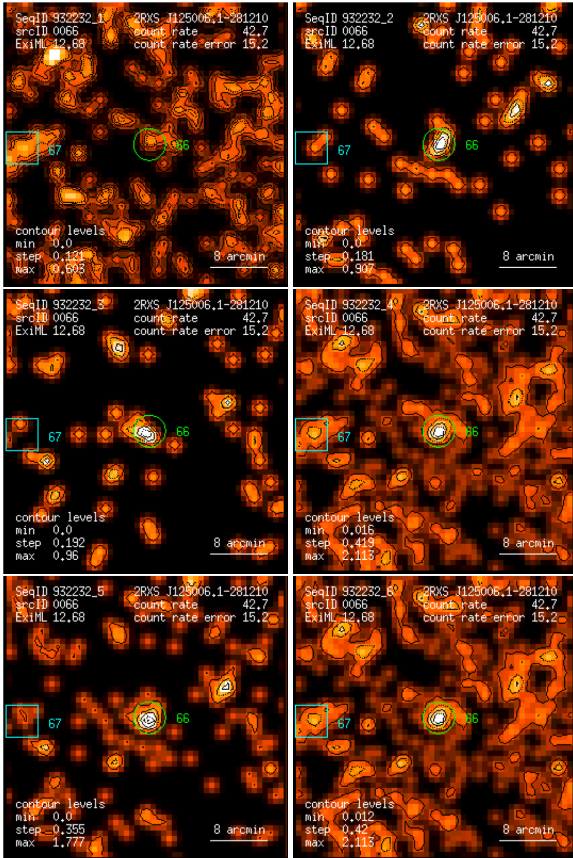
Figure 66: RASS 932232: detection 0066: band rate images, Gaussian filter: (1) PSPC channels 11 – 41, (2) 52 – 90, (3) 91 – 201, (4) 11 – 235, (5) 52 – 201, (6) 11 – 201. Broad band rates in counts/ks. Band rate contour levels in counts/ks/arcmin 2 .
