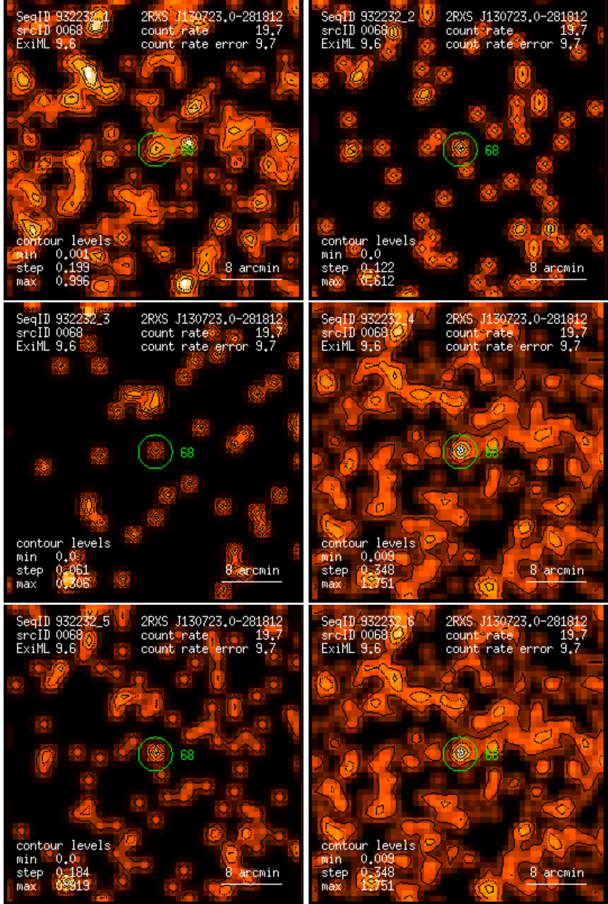
Figure 68: RASS 932232: detection 0068: band rate images, Gaussian filter: (1) PSPC channels 11 – 41, (2) 52 – 90, (3) 91 – 201, (4) 11 – 235, (5) 52 – 201, (6) 11 – 201. Broad band rates in counts/ks. Band rate contour levels in counts/ks/arcmin 2 .
