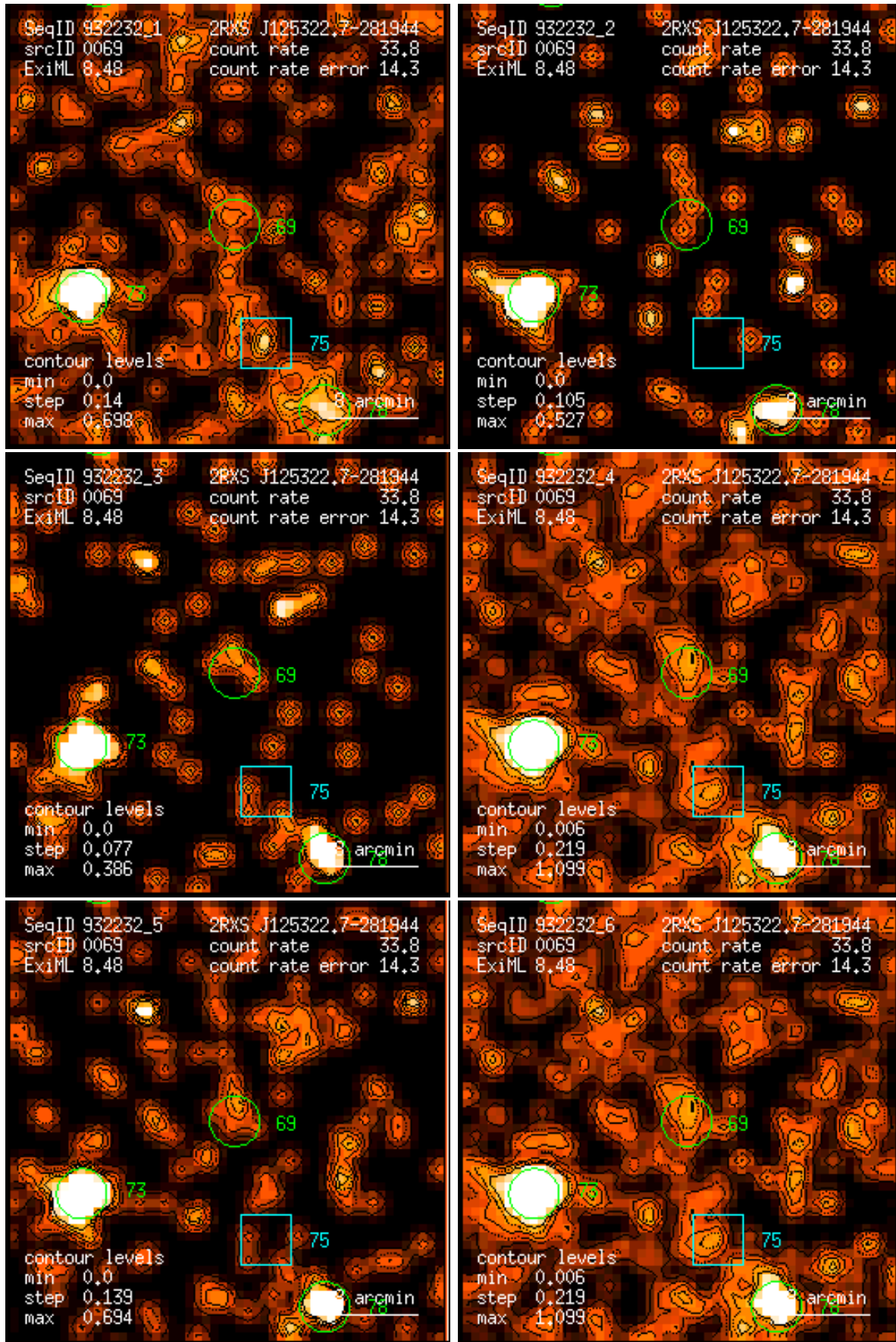
Figure 69: RASS 932232: detection 0069: band rate images, Gaussian filter: (1) PSPC channels 11 – 41, (2) 52 – 90, (3) 91 – 201, (4) 11 – 235, (5) 52 – 201, (6) 11 – 201. Broad band rates in counts/ks. Band rate contour levels in counts/ks/arcmin 2 .
