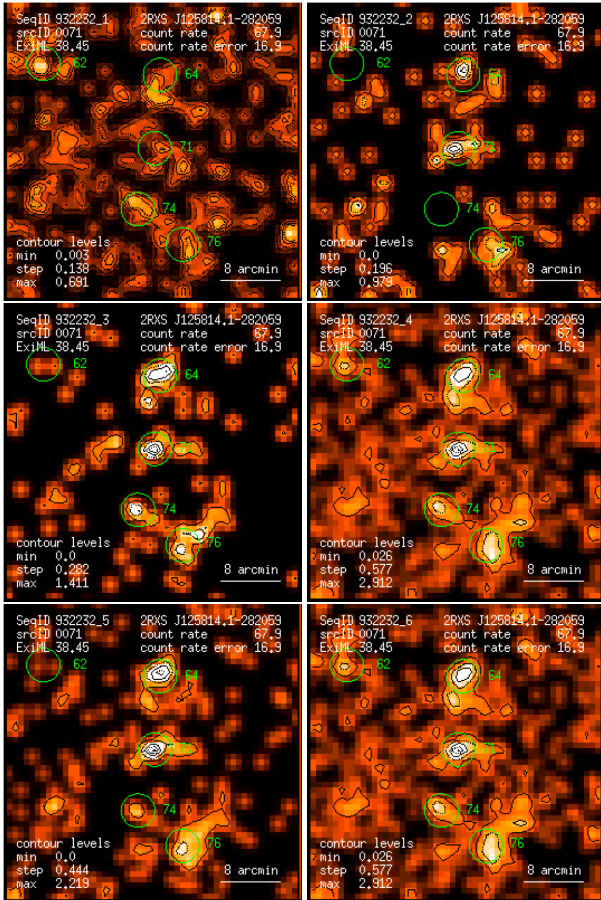
Figure 71: RASS 932232: detection 0071: band rate images, Gaussian filter: (1) PSPC channels 11 – 41, (2) 52 – 90, (3) 91 – 201, (4) 11 – 235, (5) 52 – 201, (6) 11 – 201. Broad band rates in counts/ks. Band rate contour levels in counts/ks/arcmin 2 .
