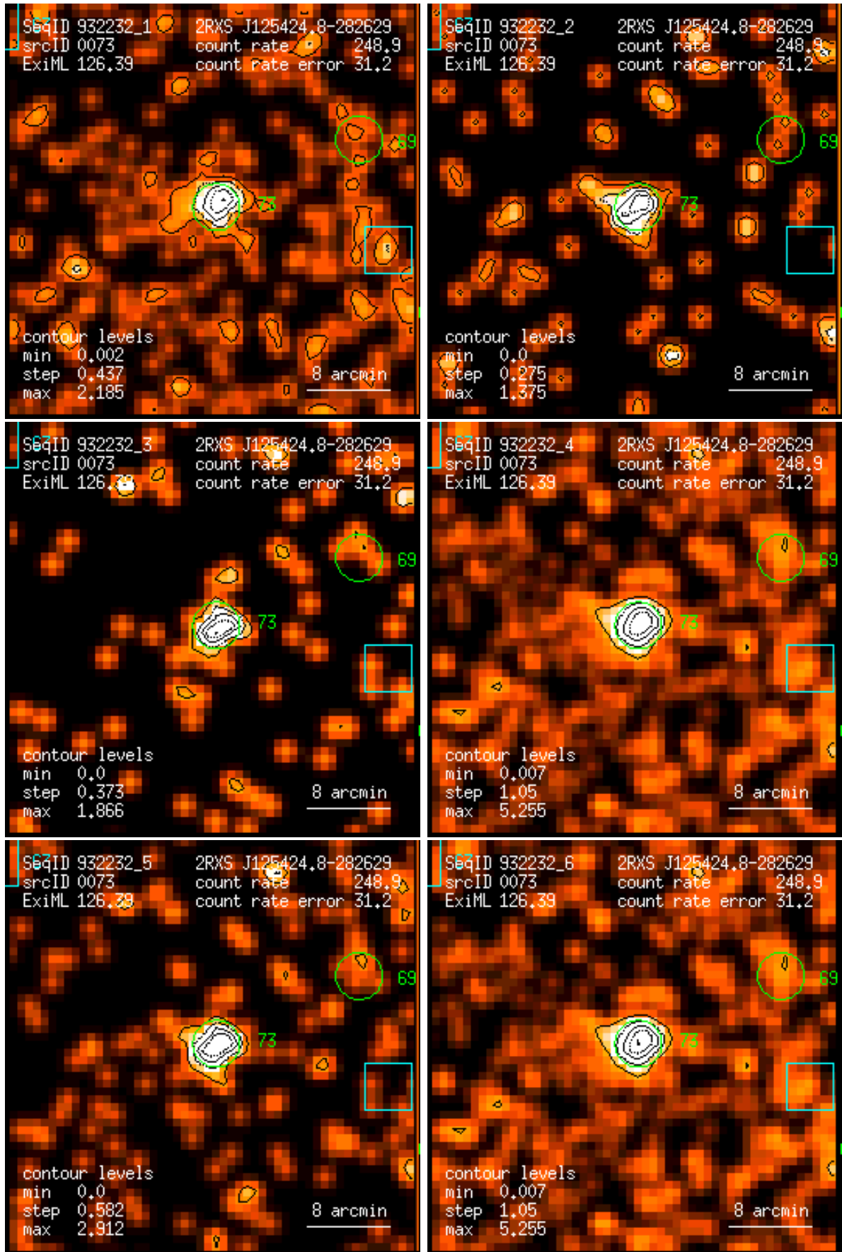
Figure 73: RASS 932232: detection 0073: band rate images, Gaussian filter: (1) PSPC channels 11 – 41, (2) 52 – 90, (3) 91 – 201, (4) 11 – 235, (5) 52 – 201, (6) 11 – 201. Broad band rates in counts/ks. Band rate contour levels in counts/ks/arcmin 2 .
